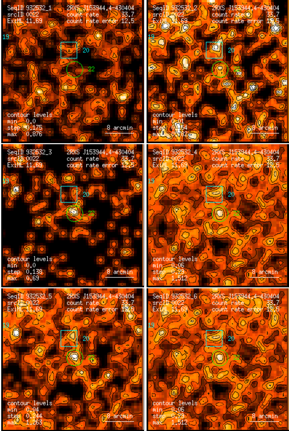
Figure 22: RASS 932532: detection 0022: band rate images, Gaussian filter: (1) PSPC channels 11 – 41, (2) 52 – 90, (3) 91 – 201, (4) 11 – 235, (5) 52 – 201, (6) 11 – 201. Broad band rates in counts/ks. Band rate contour levels in counts/ks/arcmin 2 .
