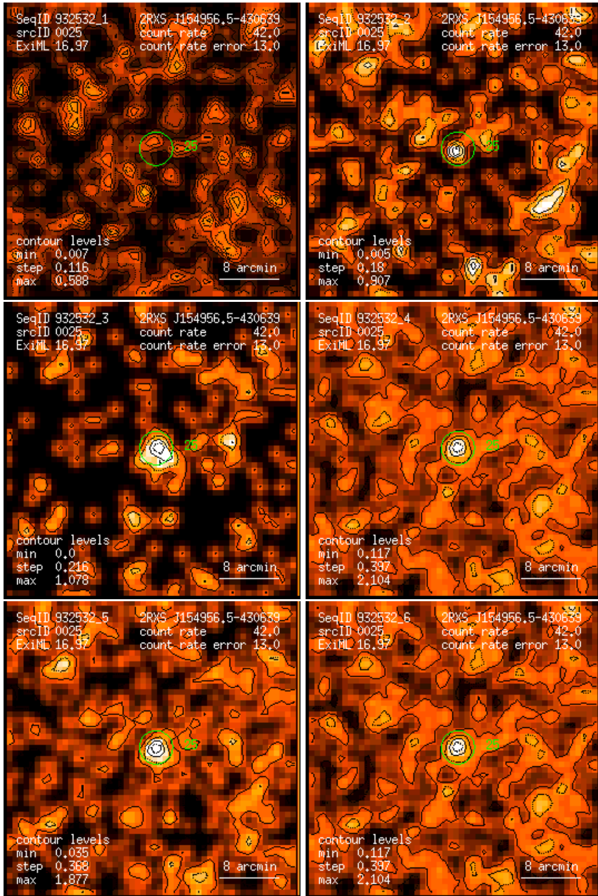
Figure 25: RASS 932532: detection 0025: band rate images, Gaussian filter: (1) PSPC channels 11 – 41, (2) 52 – 90, (3) 91 – 201, (4) 11 – 235, (5) 52 – 201, (6) 11 – 201. Broad band rates in counts/ks. Band rate contour levels in counts/ks/arcmin 2 .
