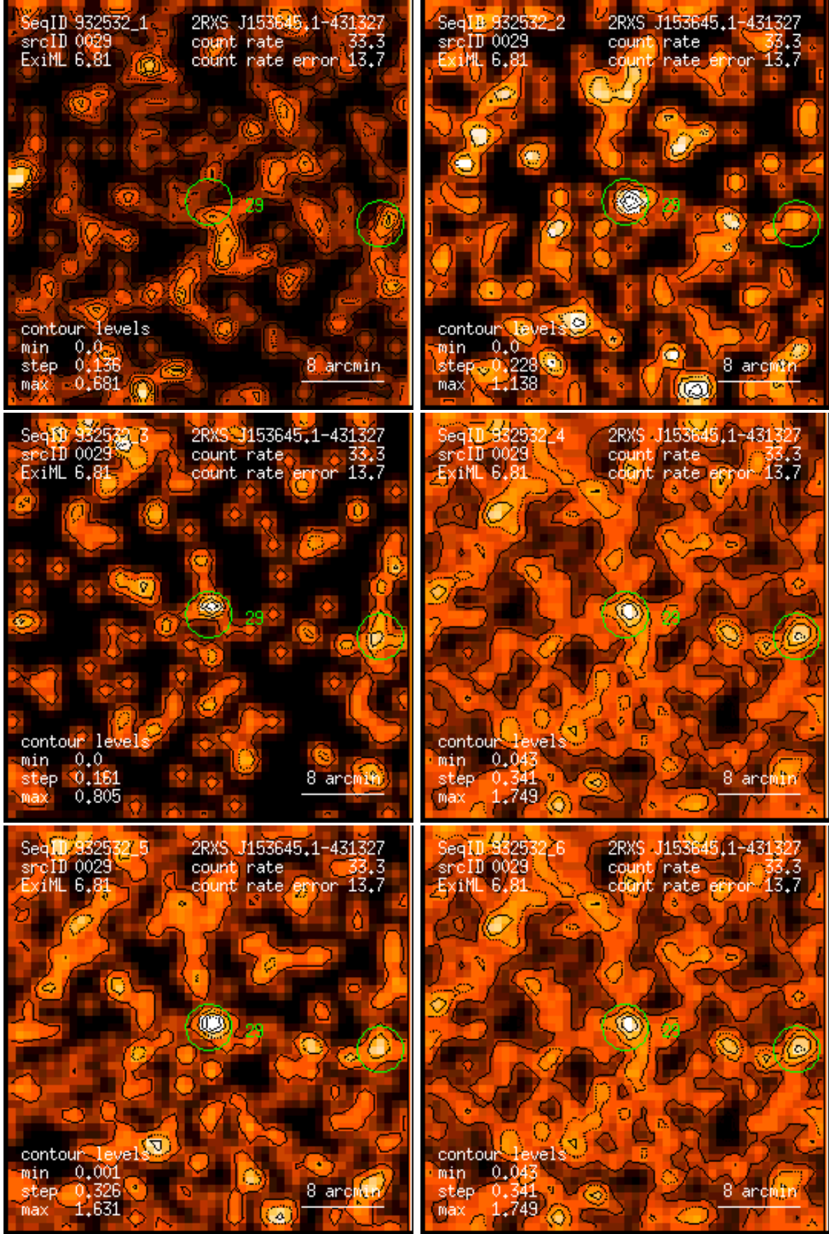
Figure 29: RASS 932532: detection 0029: band rate images, Gaussian filter: (1) PSPC channels 11 – 41, (2) 52 – 90, (3) 91 – 201, (4) 11 – 235, (5) 52 – 201, (6) 11 – 201. Broad band rates in counts/ks. Band rate contour levels in counts/ks/arcmin 2 .
