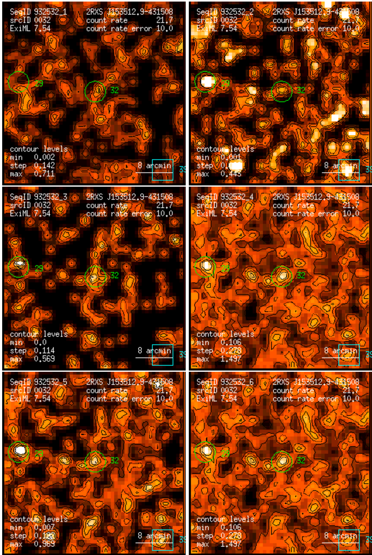
Figure 32: RASS 932532: detection 0032: band rate images, Gaussian filter: (1) PSPC channels 11 – 41, (2) 52 – 90, (3) 91 – 201, (4) 11 – 235, (5) 52 – 201, (6) 11 – 201. Broad band rates in counts/ks. Band rate contour levels in counts/ks/arcmin 2 .
