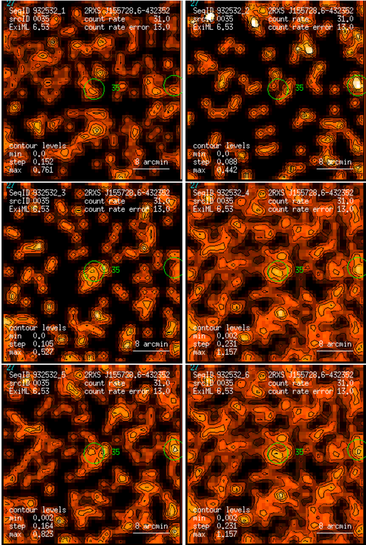
Figure 35: RASS 932532: detection 0035: band rate images, Gaussian filter: (1) PSPC channels 11 – 41, (2) 52 – 90, (3) 91 – 201, (4) 11 – 235, (5) 52 – 201, (6) 11 – 201. Broad band rates in counts/ks. Band rate contour levels in counts/ks/arcmin 2 .
