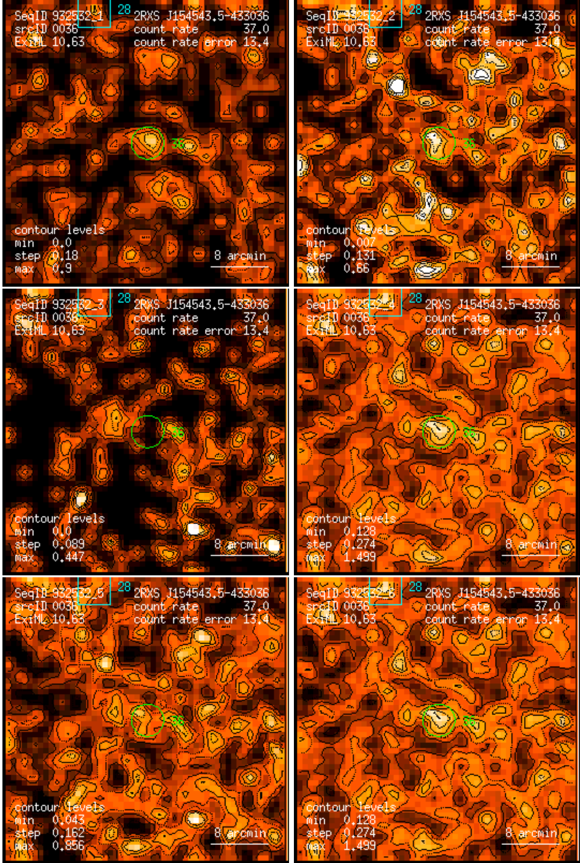
Figure 36: RASS 932532: detection 0036: band rate images, Gaussian filter: (1) PSPC channels 11 – 41, (2) 52 – 90, (3) 91 – 201, (4) 11 – 235, (5) 52 – 201, (6) 11 – 201. Broad band rates in counts/ks. Band rate contour levels in counts/ks/arcmin 2 .
