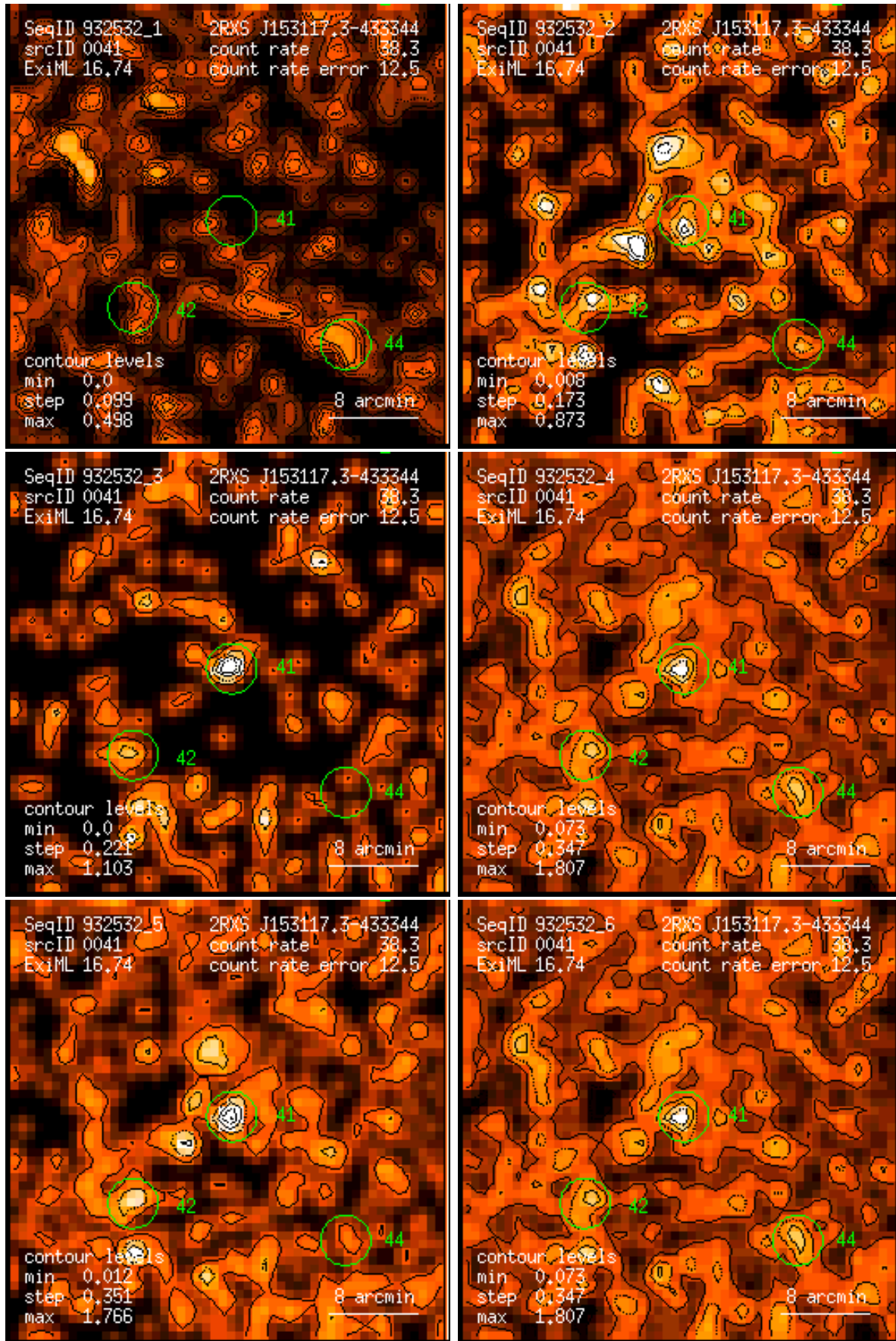
Figure 41: RASS 932532: detection 0041: band rate images, Gaussian filter: (1) PSPC channels 11 – 41, (2) 52 – 90, (3) 91 – 201, (4) 11 – 235, (5) 52 – 201, (6) 11 – 201. Broad band rates in counts/ks. Band rate contour levels in counts/ks/arcmin 2 .
