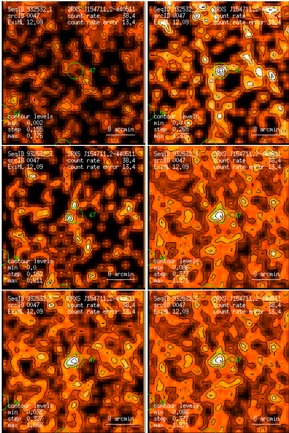
Figure 47: RASS 932532: detection 0047: band rate images, Gaussian filter: (1) PSPC channels 11 – 41, (2) 52 – 90, (3) 91 – 201, (4) 11 – 235, (5) 52 – 201, (6) 11 – 201. Broad band rates in counts/ks. Band rate contour levels in counts/ks/arcmin 2 .
