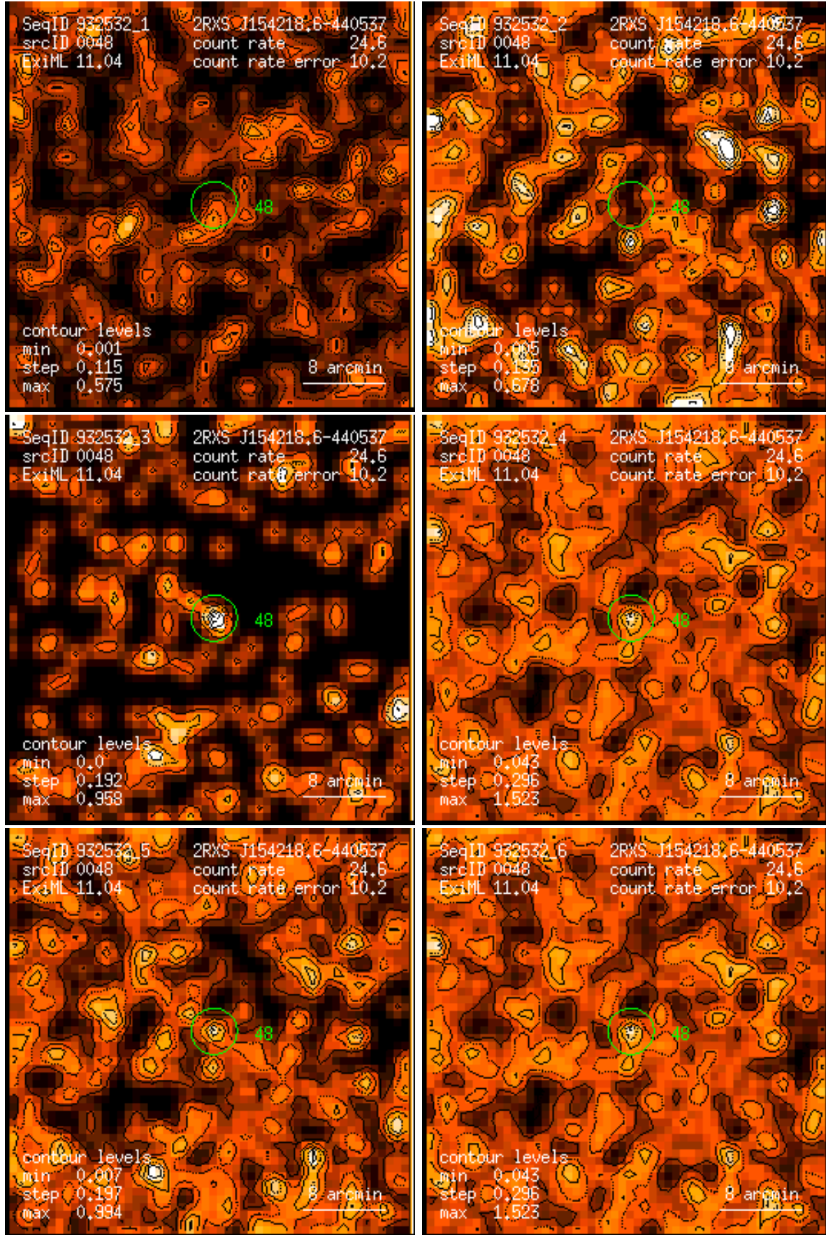
Figure 48: RASS 932532: detection 0048: band rate images, Gaussian filter: (1) PSPC channels 11 – 41, (2) 52 – 90, (3) 91 – 201, (4) 11 – 235, (5) 52 – 201, (6) 11 – 201. Broad band rates in counts/ks. Band rate contour levels in counts/ks/arcmin 2 .
