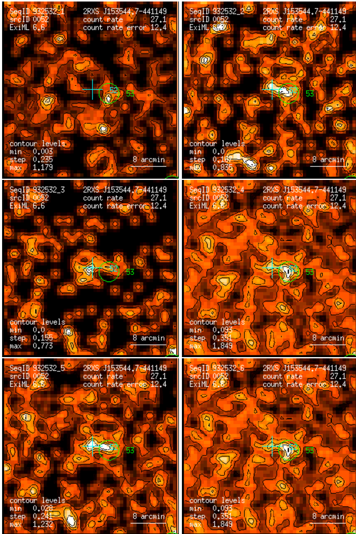
Figure 52: RASS 932532: detection 0052: band rate images, Gaussian filter: (1) PSPC channels 11 – 41, (2) 52 – 90, (3) 91 – 201, (4) 11 – 235, (5) 52 – 201, (6) 11 – 201. Broad band rates in counts/ks. Band rate contour levels in counts/ks/arcmin 2 .
