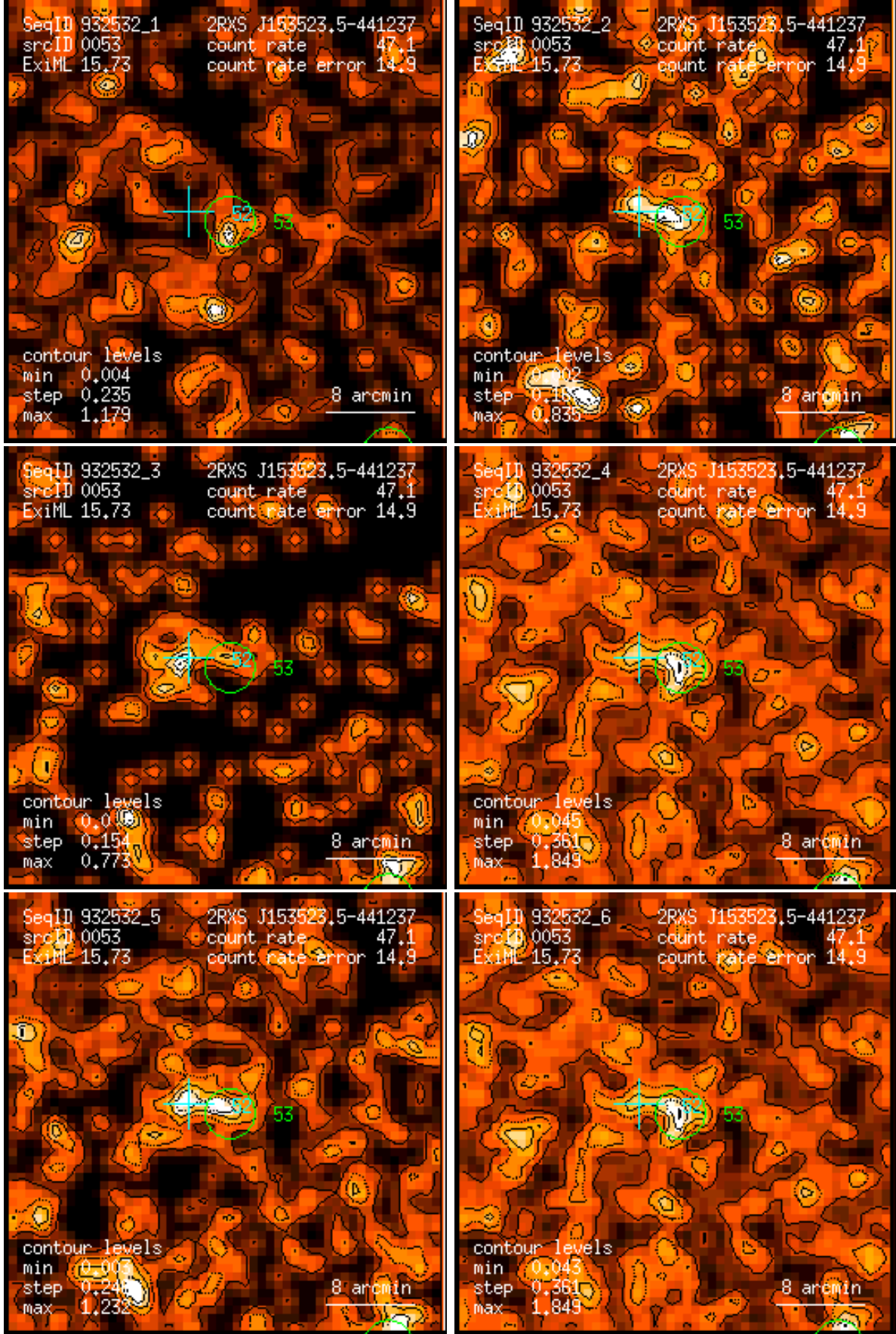
Figure 53: RASS 932532: detection 0053: band rate images, Gaussian filter: (1) PSPC channels 11 – 41, (2) 52 – 90, (3) 91 – 201, (4) 11 – 235, (5) 52 – 201, (6) 11 – 201. Broad band rates in counts/ks. Band rate contour levels in counts/ks/arcmin 2 .
