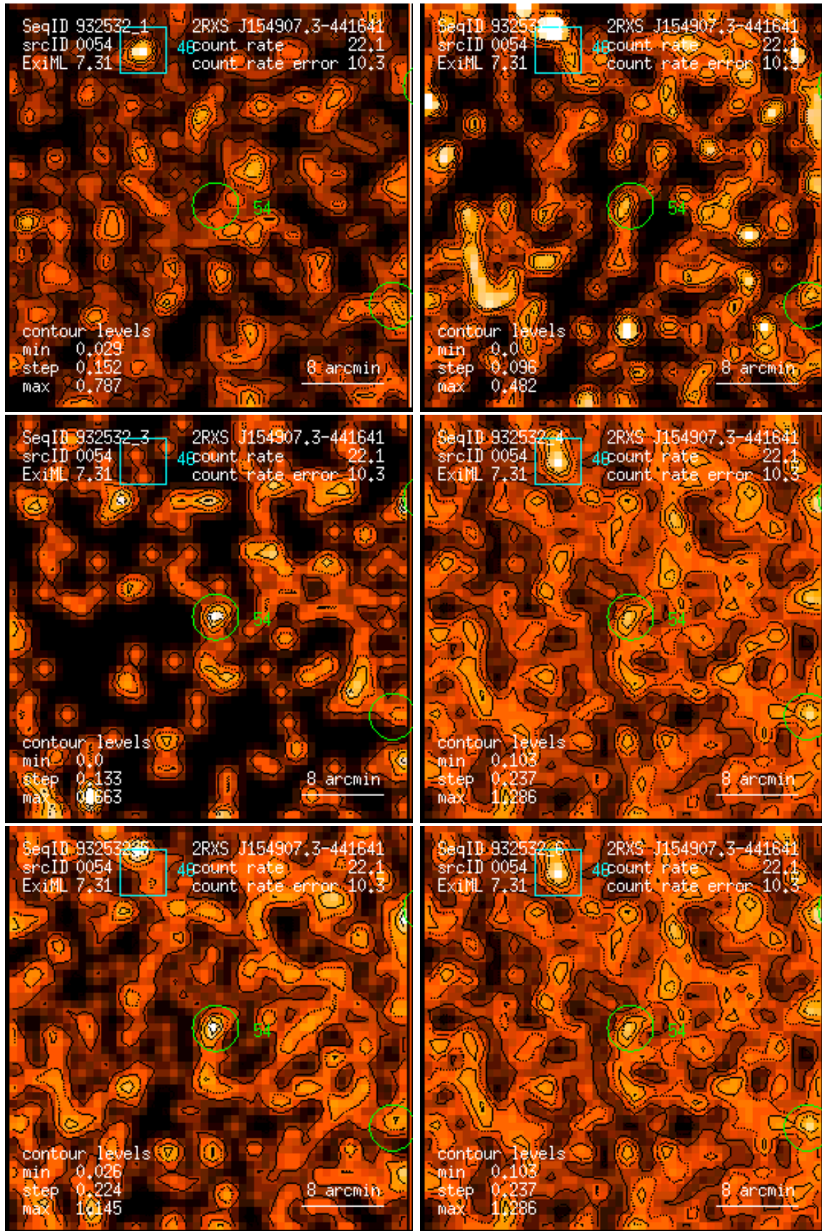
Figure 54: RASS 932532: detection 0054: band rate images, Gaussian filter: (1) PSPC channels 11 – 41, (2) 52 – 90, (3) 91 – 201, (4) 11 – 235, (5) 52 – 201, (6) 11 – 201. Broad band rates in counts/ks. Band rate contour levels in counts/ks/arcmin 2 .
