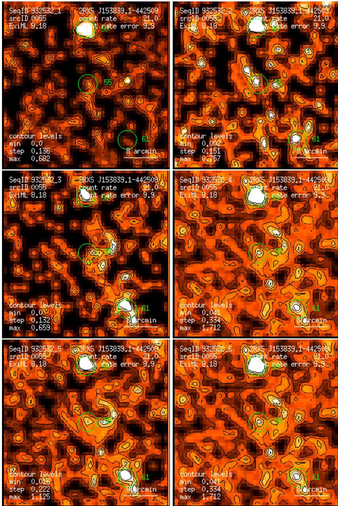
Figure 55: RASS 932532: detection 0055: band rate images, Gaussian filter: (1) PSPC channels 11 – 41, (2) 52 – 90, (3) 91 – 201, (4) 11 – 235, (5) 52 – 201, (6) 11 – 201. Broad band rates in counts/ks. Band rate contour levels in counts/ks/arcmin 2 .
