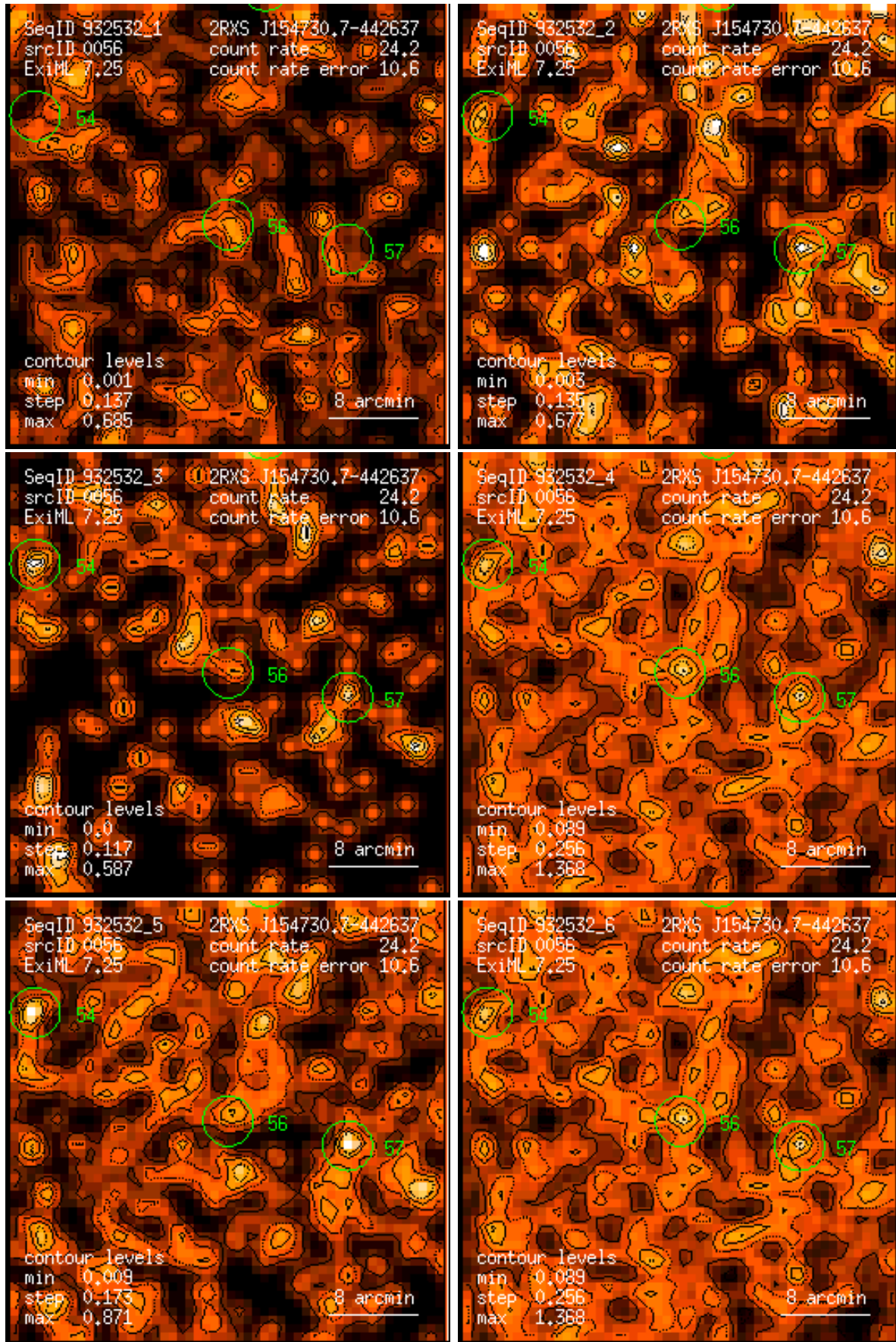
Figure 56: RASS 932532: detection 0056: band rate images, Gaussian filter: (1) PSPC channels 11 – 41, (2) 52 – 90, (3) 91 – 201, (4) 11 – 235, (5) 52 – 201, (6) 11 – 201. Broad band rates in counts/ks. Band rate contour levels in counts/ks/arcmin 2 .
