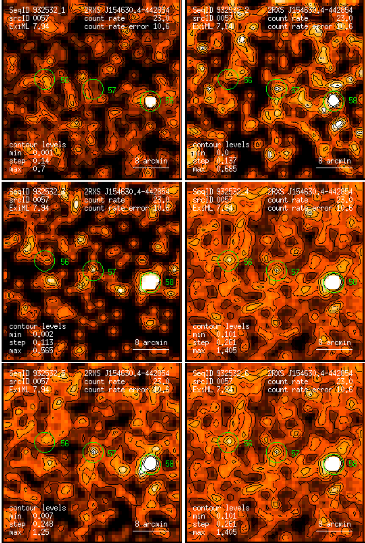
Figure 57: RASS 932532: detection 0057: band rate images, Gaussian filter: (1) PSPC channels 11 – 41, (2) 52 – 90, (3) 91 – 201, (4) 11 – 235, (5) 52 – 201, (6) 11 – 201. Broad band rates in counts/ks. Band rate contour levels in counts/ks/arcmin 2 .
