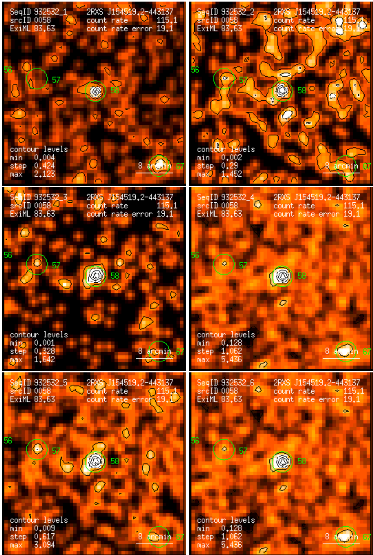
Figure 58: RASS 932532: detection 0058: band rate images, Gaussian filter: (1) PSPC channels 11 – 41, (2) 52 – 90, (3) 91 – 201, (4) 11 – 235, (5) 52 – 201, (6) 11 – 201. Broad band rates in counts/ks. Band rate contour levels in counts/ks/arcmin 2 .
