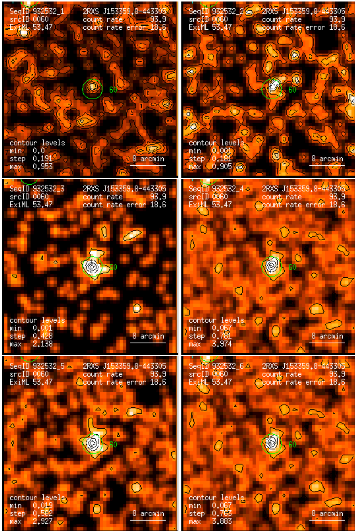
Figure 60: RASS 932532: detection 0060: band rate images, Gaussian filter: (1) PSPC channels 11 – 41, (2) 52 – 90, (3) 91 – 201, (4) 11 – 235, (5) 52 – 201, (6) 11 – 201. Broad band rates in counts/ks. Band rate contour levels in counts/ks/arcmin 2 .
