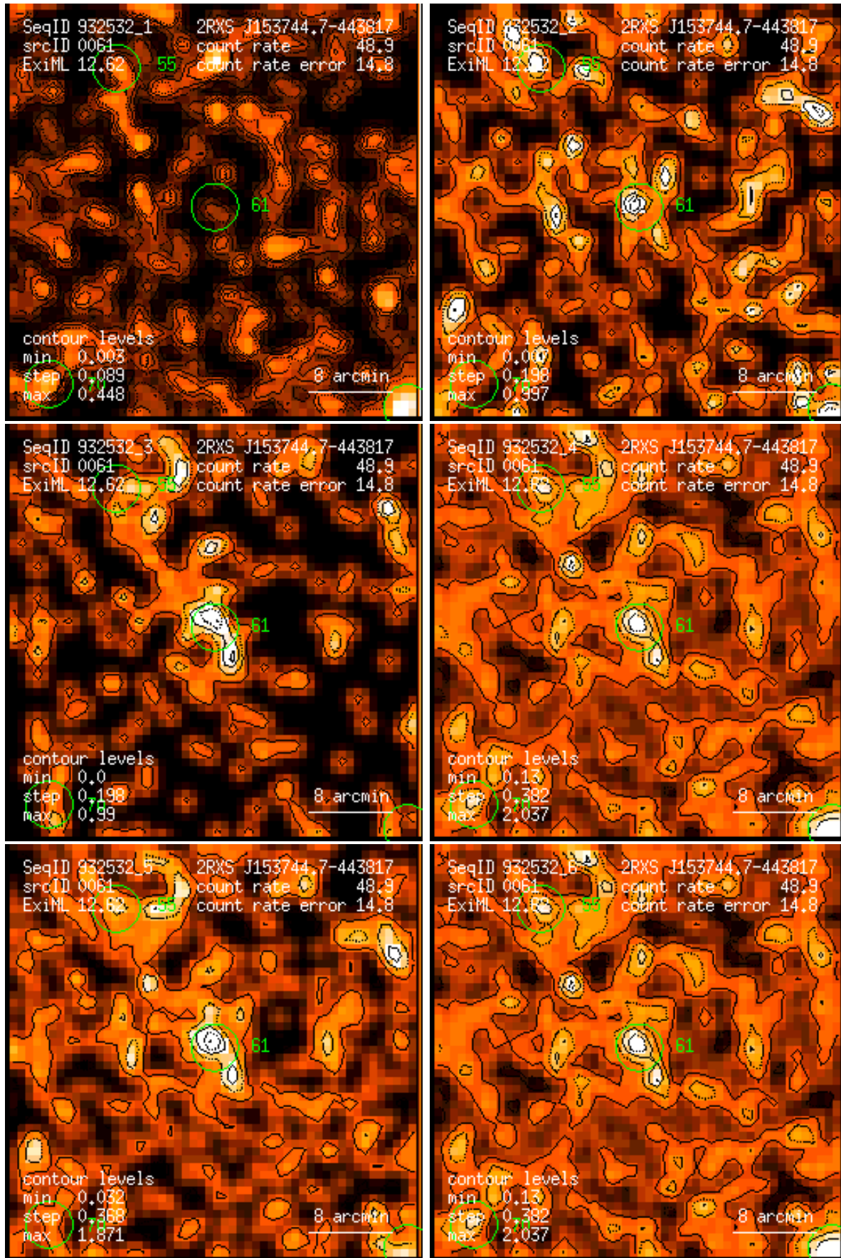
Figure 61: RASS 932532: detection 0061: band rate images, Gaussian filter: (1) PSPC channels 11 – 41, (2) 52 – 90, (3) 91 – 201, (4) 11 – 235, (5) 52 – 201, (6) 11 – 201. Broad band rates in counts/ks. Band rate contour levels in counts/ks/arcmin 2 .
