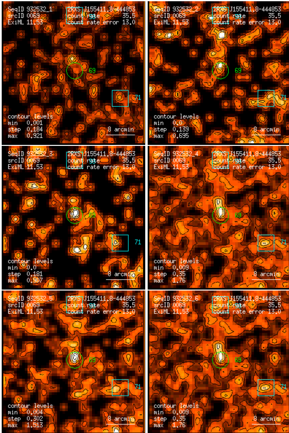
Figure 69: RASS 932532: detection 0069: band rate images, Gaussian filter: (1) PSPC channels 11 – 41, (2) 52 – 90, (3) 91 – 201, (4) 11 – 235, (5) 52 – 201, (6) 11 – 201. Broad band rates in counts/ks. Band rate contour levels in counts/ks/arcmin 2 .
