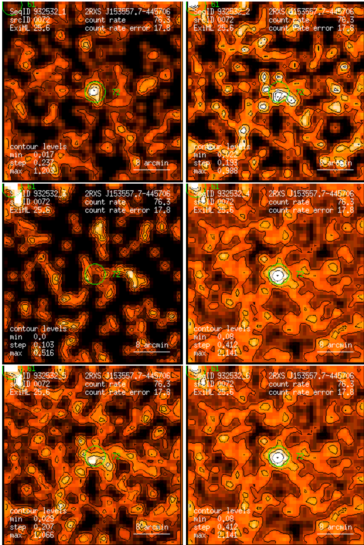
Figure 72: RASS 932532: detection 0072: band rate images, Gaussian filter: (1) PSPC channels 11 – 41, (2) 52 – 90, (3) 91 – 201, (4) 11 – 235, (5) 52 – 201, (6) 11 – 201. Broad band rates in counts/ks. Band rate contour levels in counts/ks/arcmin 2 .
