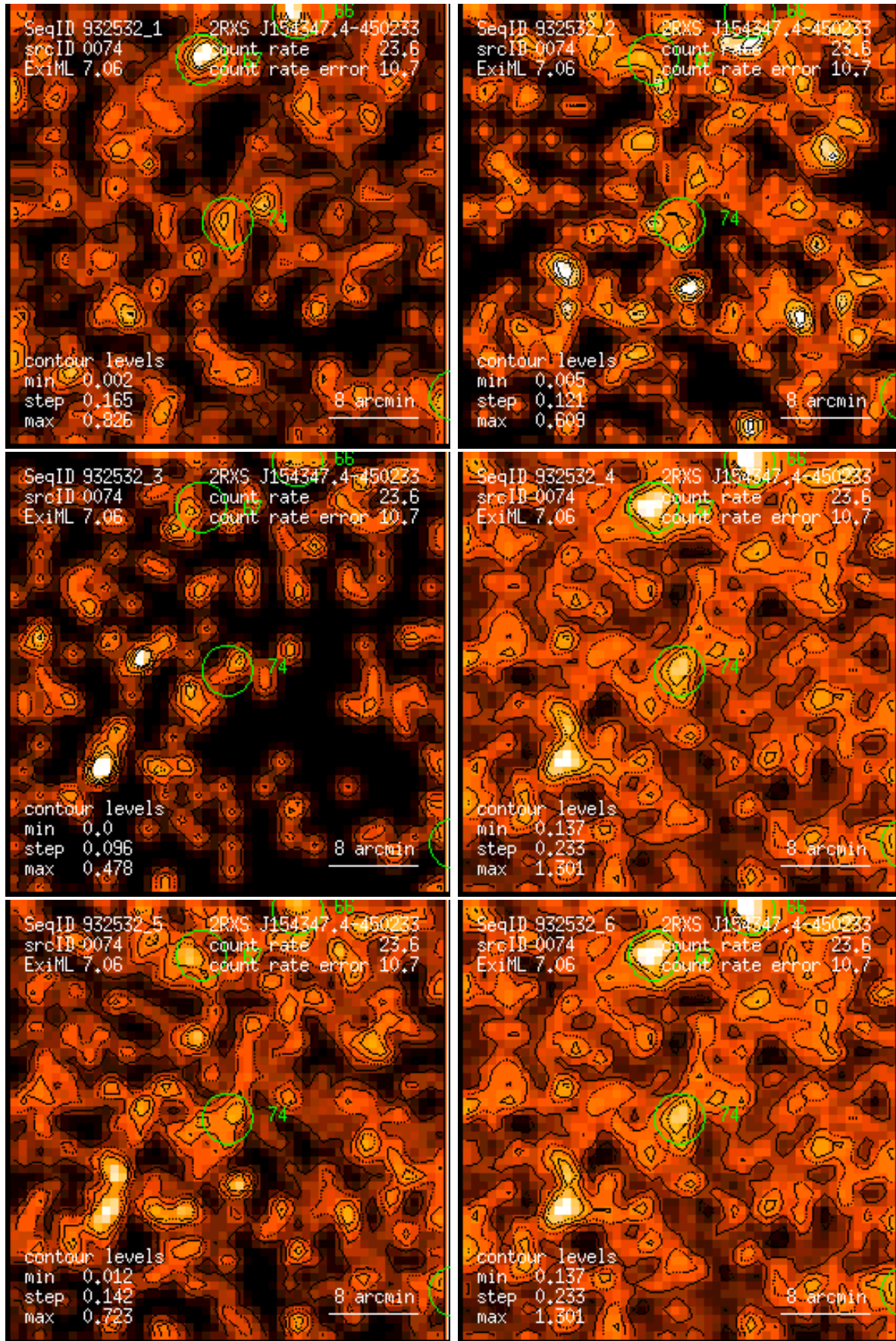
Figure 74: RASS 932532: detection 0074: band rate images, Gaussian filter: (1) PSPC channels 11 – 41, (2) 52 – 90, (3) 91 – 201, (4) 11 – 235, (5) 52 – 201, (6) 11 – 201. Broad band rates in counts/ks. Band rate contour levels in counts/ks/arcmin 2 .
