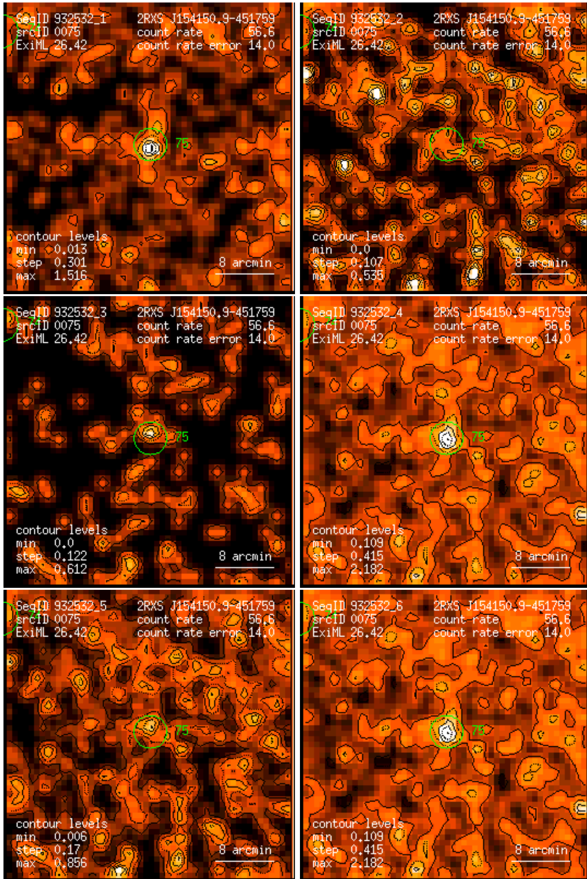
Figure 75: RASS 932532: detection 0075: band rate images, Gaussian filter: (1) PSPC channels 11 – 41, (2) 52 – 90, (3) 91 – 201, (4) 11 – 235, (5) 52 – 201, (6) 11 – 201. Broad band rates in counts/ks. Band rate contour levels in counts/ks/arcmin 2 .
