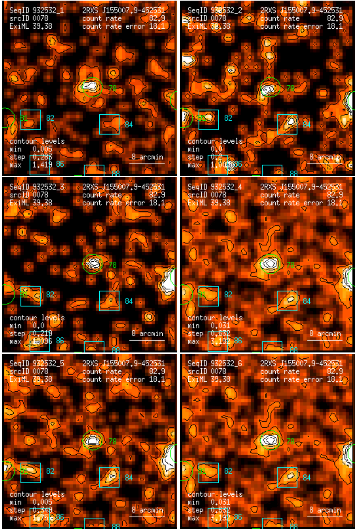
Figure 78: RASS 932532: detection 0078: band rate images, Gaussian filter: (1) PSPC channels 11 – 41, (2) 52 – 90, (3) 91 – 201, (4) 11 – 235, (5) 52 – 201, (6) 11 – 201. Broad band rates in counts/ks. Band rate contour levels in counts/ks/arcmin 2 .
