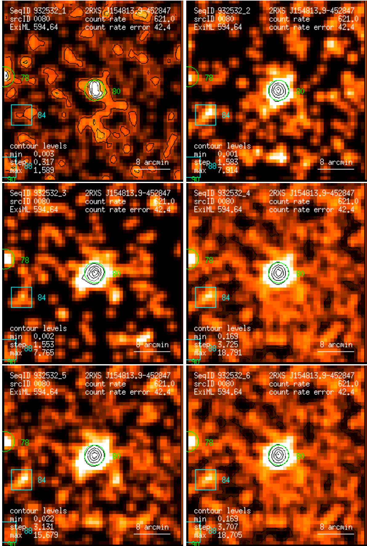
Figure 80: RASS 932532: detection 0080: band rate images, Gaussian filter: (1) PSPC channels 11 – 41, (2) 52 – 90, (3) 91 – 201, (4) 11 – 235, (5) 52 – 201, (6) 11 – 201. Broad band rates in counts/ks. Band rate contour levels in counts/ks/arcmin 2 .
