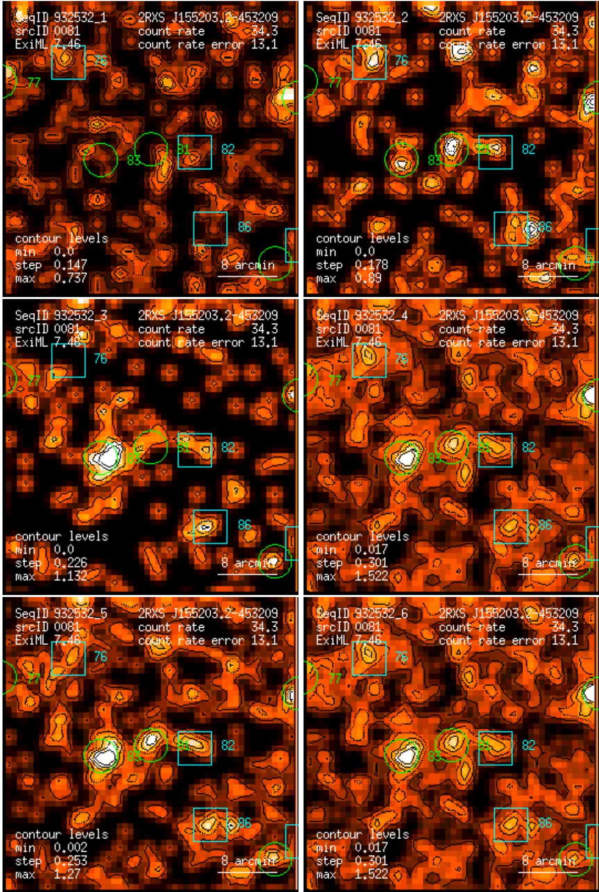
Figure 81: RASS 932532: detection 0081: band rate images, Gaussian filter: (1) PSPC channels 11 – 41, (2) 52 – 90, (3) 91 – 201, (4) 11 – 235, (5) 52 – 201, (6) 11 – 201. Broad band rates in counts/ks. Band rate contour levels in counts/ks/arcmin 2 .
