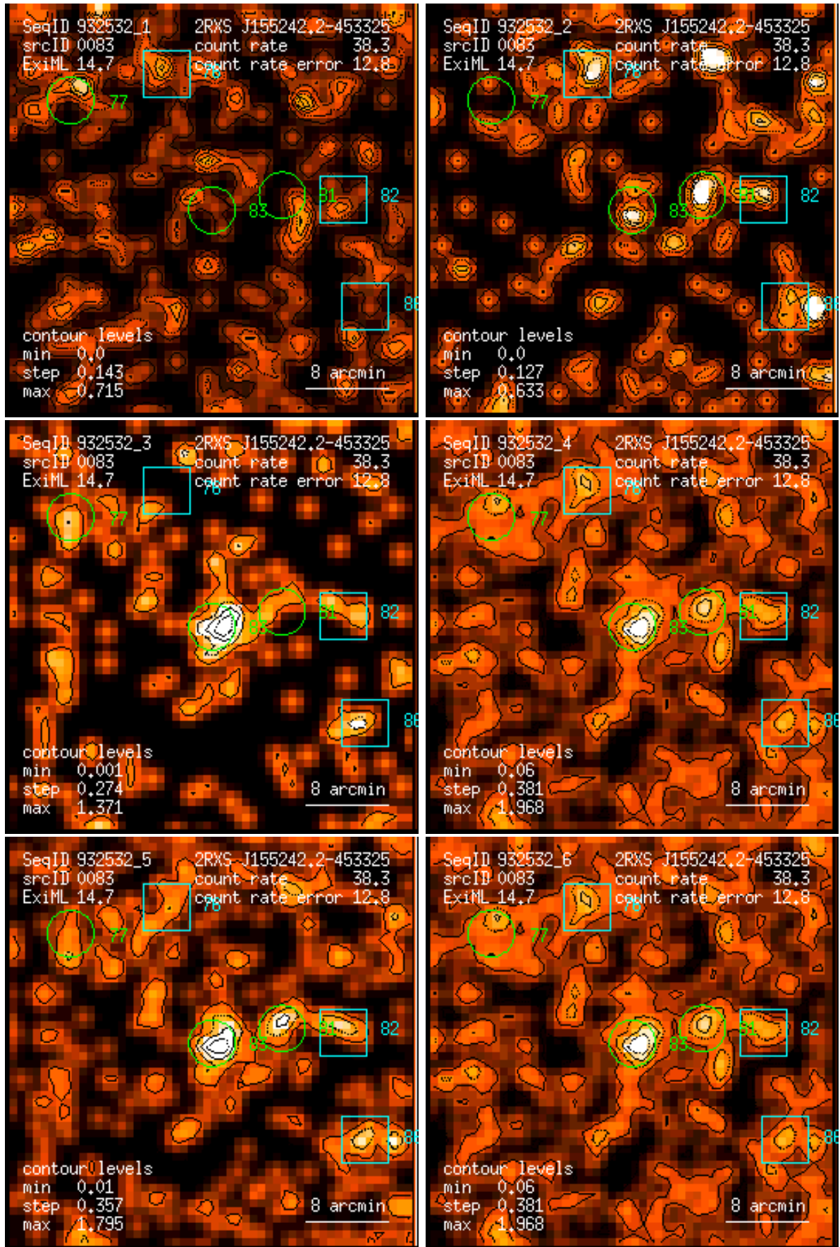
Figure 83: RASS 932532: detection 0083: band rate images, Gaussian filter: (1) PSPC channels 11 – 41, (2) 52 – 90, (3) 91 – 201, (4) 11 – 235, (5) 52 – 201, (6) 11 – 201. Broad band rates in counts/ks. Band rate contour levels in counts/ks/arcmin 2 .
