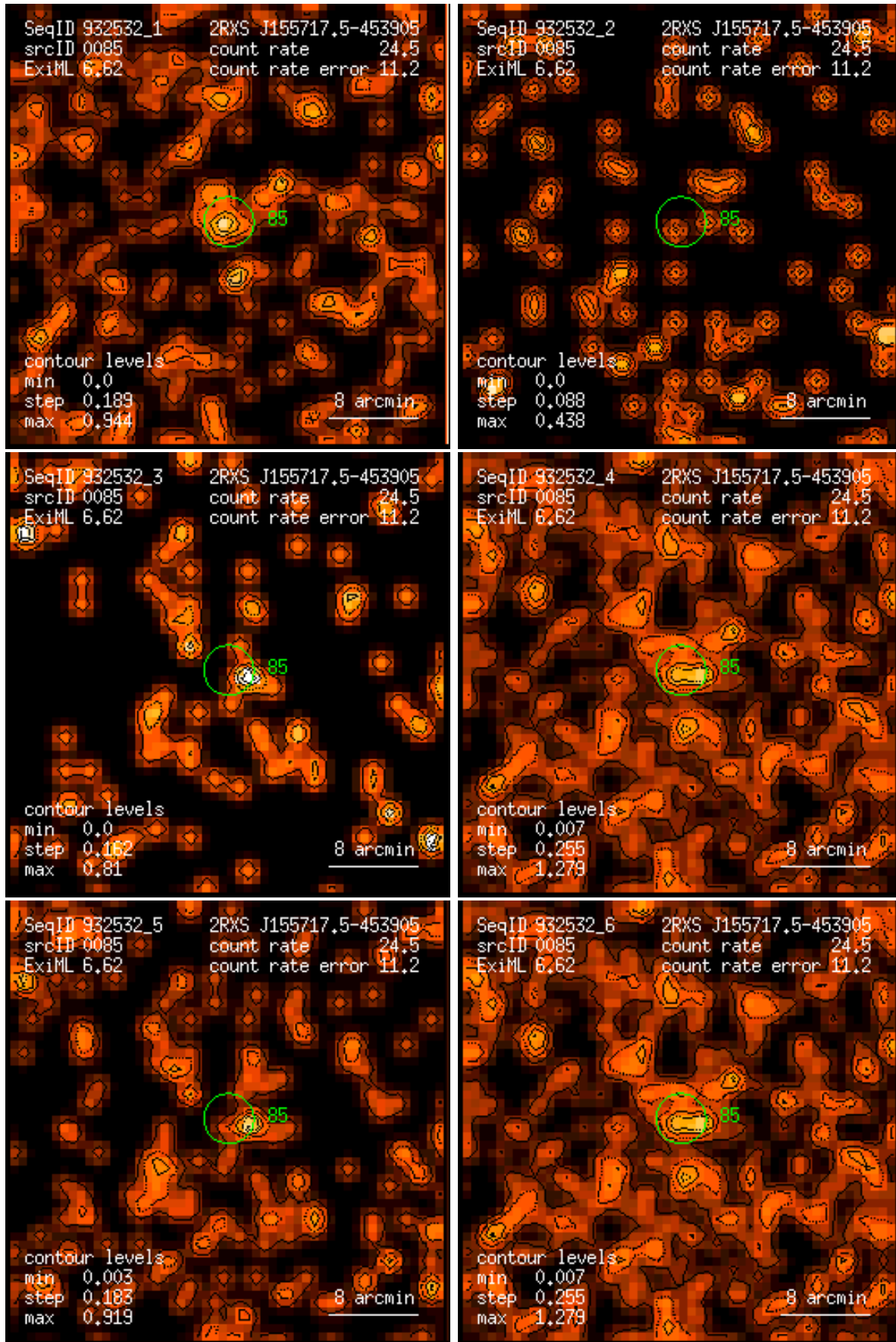
Figure 85: RASS 932532: detection 0085: band rate images, Gaussian filter: (1) PSPC channels 11 – 41, (2) 52 – 90, (3) 91 – 201, (4) 11 – 235, (5) 52 – 201, (6) 11 – 201. Broad band rates in counts/ks. Band rate contour levels in counts/ks/arcmin 2 .
