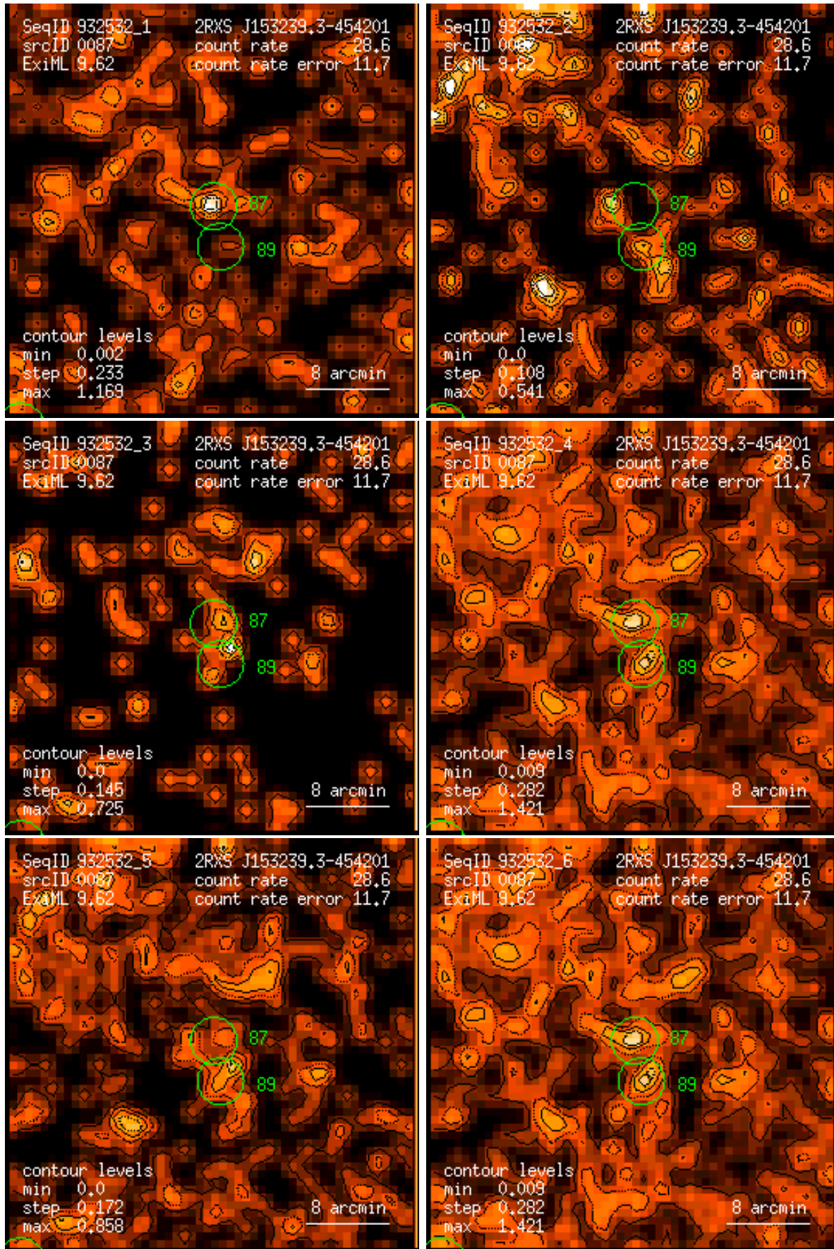
Figure 87: RASS 932532: detection 0087: band rate images, Gaussian filter: (1) PSPC channels 11 – 41, (2) 52 – 90, (3) 91 – 201, (4) 11 – 235, (5) 52 – 201, (6) 11 – 201. Broad band rates in counts/ks. Band rate contour levels in counts/ks/arcmin 2 .
