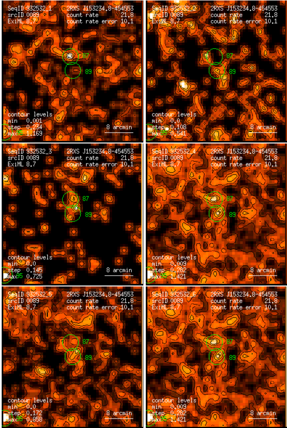
Figure 89: RASS 932532: detection 0089: band rate images, Gaussian filter: (1) PSPC channels 11 – 41, (2) 52 – 90, (3) 91 – 201, (4) 11 – 235, (5) 52 – 201, (6) 11 – 201. Broad band rates in counts/ks. Band rate contour levels in counts/ks/arcmin 2 .
