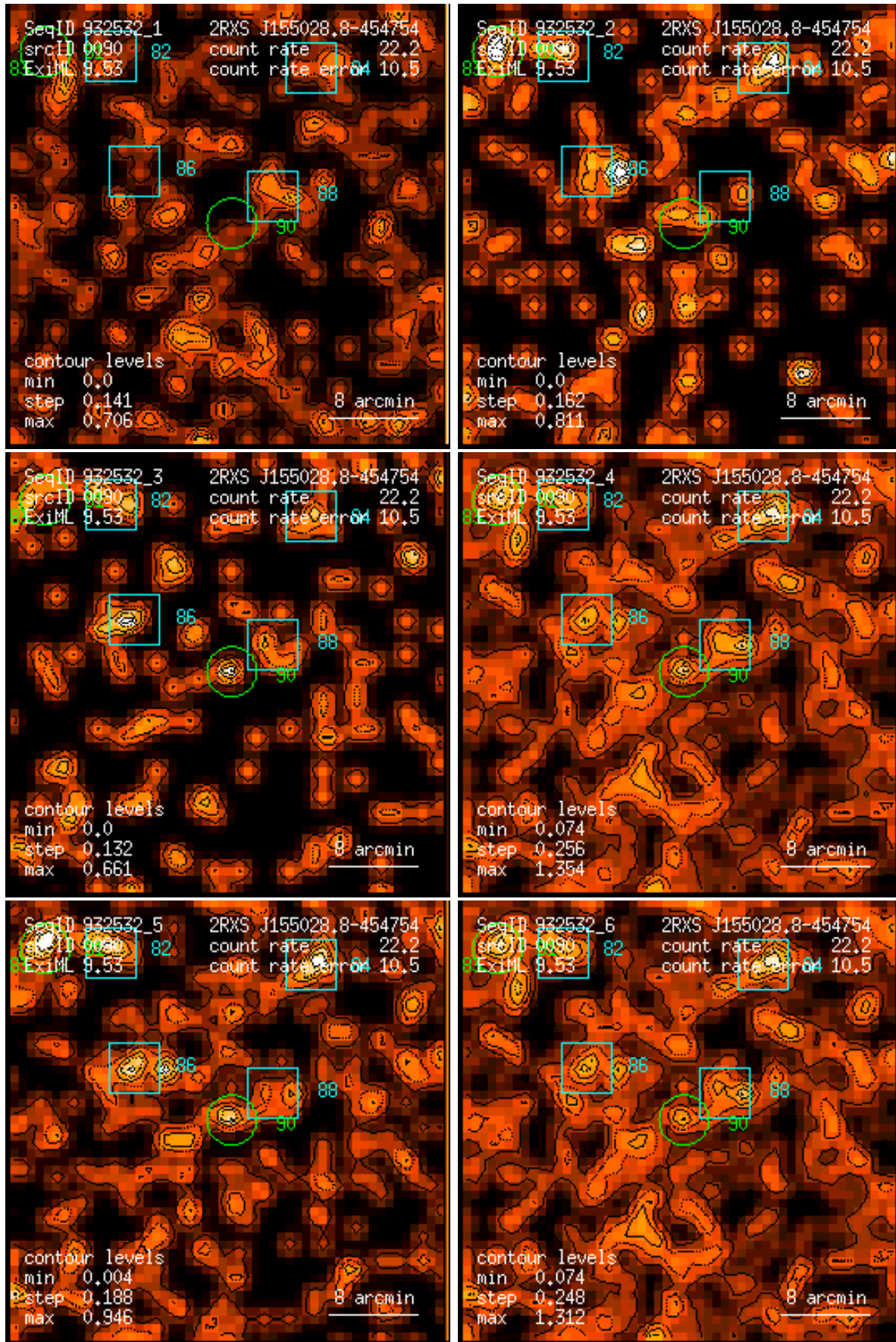
Figure 90: RASS 932532: detection 0090: band rate images, Gaussian filter: (1) PSPC channels 11 – 41, (2) 52 – 90, (3) 91 – 201, (4) 11 – 235, (5) 52 – 201, (6) 11 – 201. Broad band rates in counts/ks. Band rate contour levels in counts/ks/arcmin 2 .
