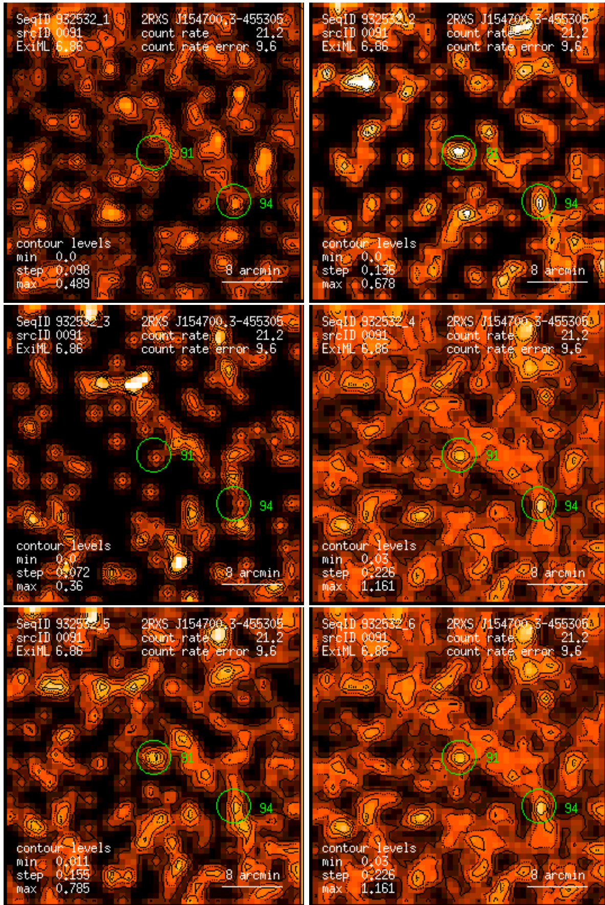
Figure 91: RASS 932532: detection 0091: band rate images, Gaussian filter: (1) PSPC channels 11 – 41, (2) 52 – 90, (3) 91 – 201, (4) 11 – 235, (5) 52 – 201, (6) 11 – 201. Broad band rates in counts/ks. Band rate contour levels in counts/ks/arcmin 2 .
