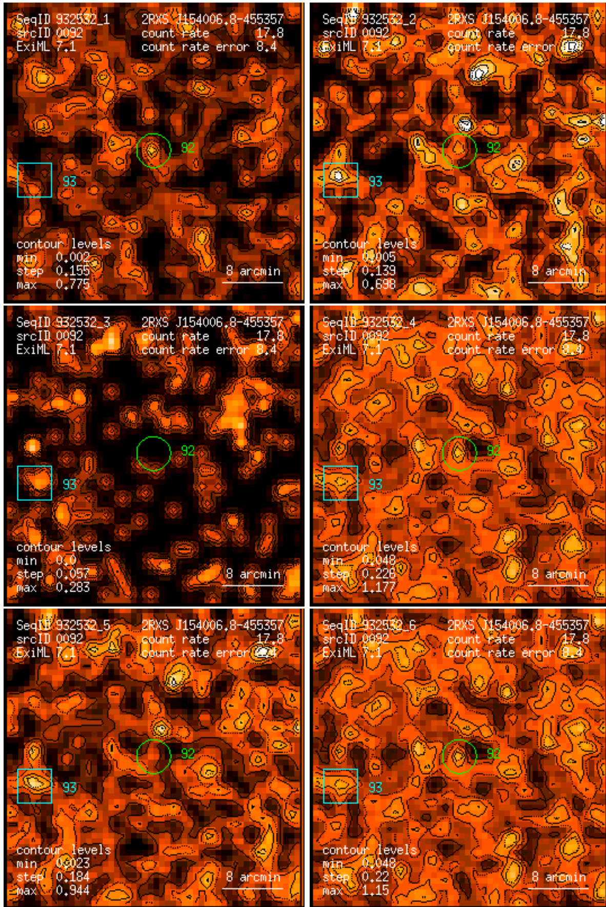
Figure 92: RASS 932532: detection 0092: band rate images, Gaussian filter: (1) PSPC channels 11 – 41, (2) 52 – 90, (3) 91 – 201, (4) 11 – 235, (5) 52 – 201, (6) 11 – 201. Broad band rates in counts/ks. Band rate contour levels in counts/ks/arcmin 2 .
