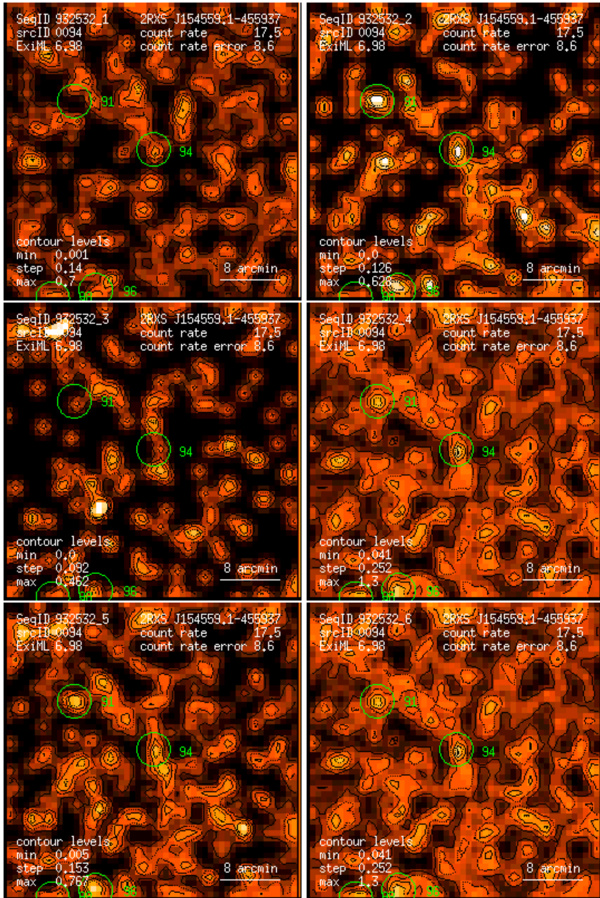
Figure 94: RASS 932532: detection 0094: band rate images, Gaussian filter: (1) PSPC channels 11 – 41, (2) 52 – 90, (3) 91 – 201, (4) 11 – 235, (5) 52 – 201, (6) 11 – 201. Broad band rates in counts/ks. Band rate contour levels in counts/ks/arcmin 2 .
