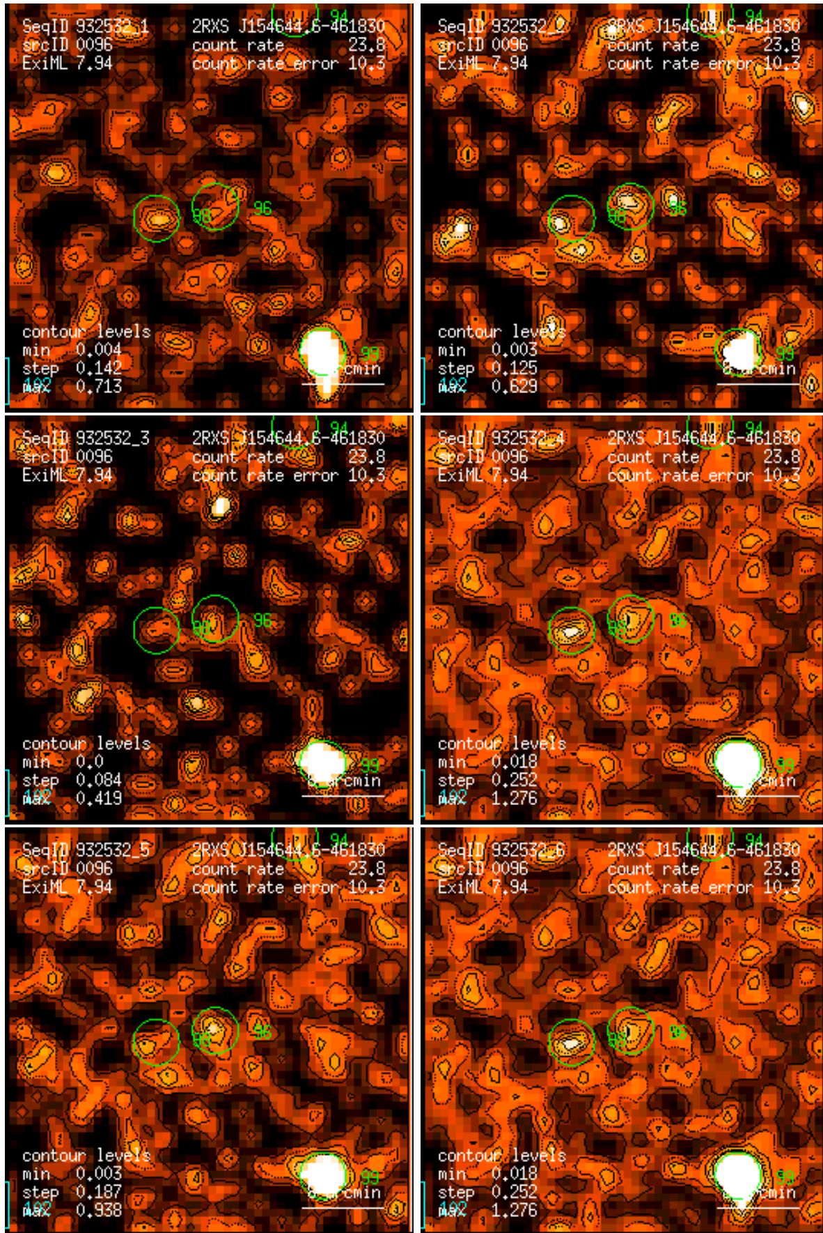
Figure 96: RASS 932532: detection 0096: band rate images, Gaussian filter: (1) PSPC channels 11 – 41, (2) 52 – 90, (3) 91 – 201, (4) 11 – 235, (5) 52 – 201, (6) 11 – 201. Broad band rates in counts/ks. Band rate contour levels in counts/ks/arcmin 2 .
