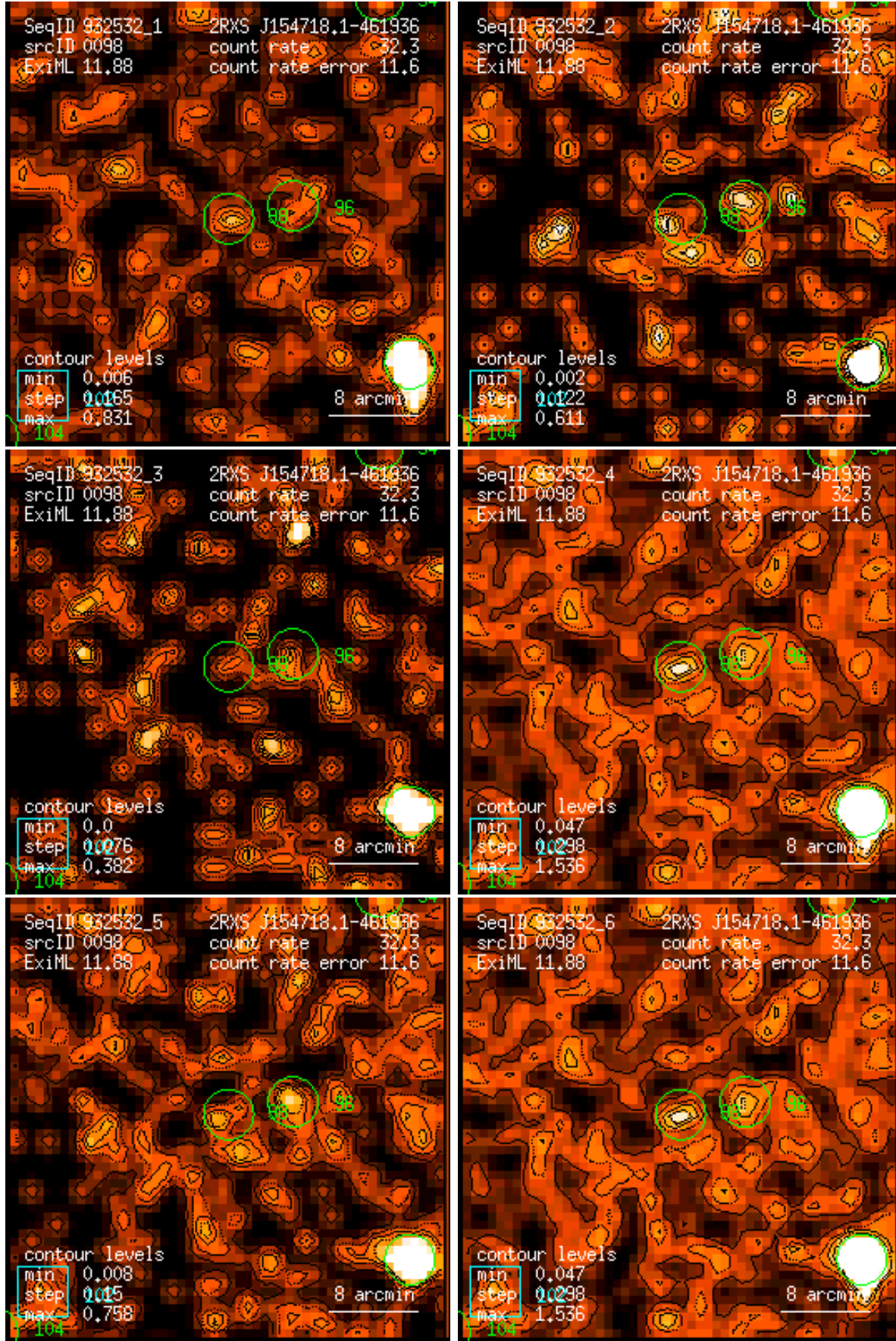
Figure 98: RASS 932532: detection 0098: band rate images, Gaussian filter: (1) PSPC channels 11 – 41, (2) 52 – 90, (3) 91 – 201, (4) 11 – 235, (5) 52 – 201, (6) 11 – 201. Broad band rates in counts/ks. Band rate contour levels in counts/ks/arcmin 2 .
