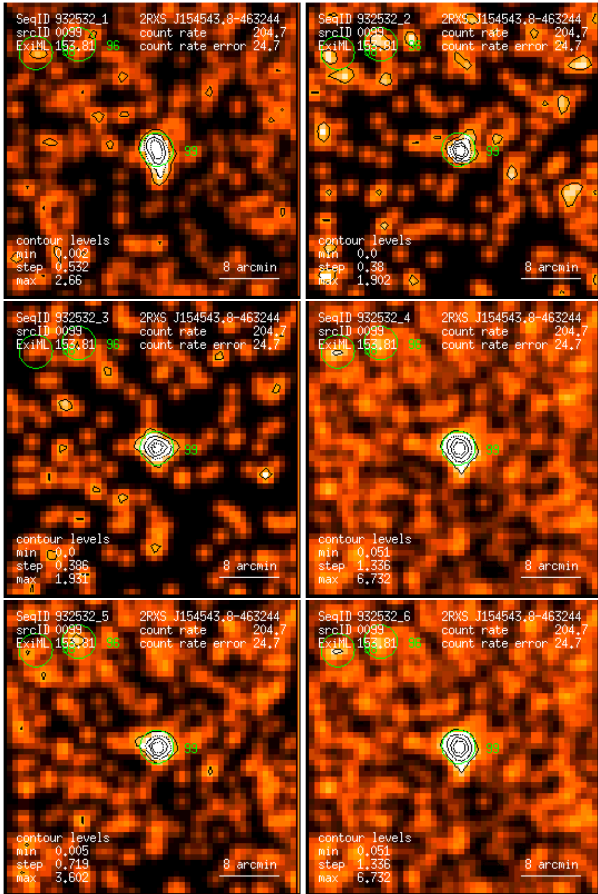
Figure 99: RASS 932532: detection 0099: band rate images, Gaussian filter: (1) PSPC channels 11 – 41, (2) 52 – 90, (3) 91 – 201, (4) 11 – 235, (5) 52 – 201, (6) 11 – 201. Broad band rates in counts/ks. Band rate contour levels in counts/ks/arcmin 2 .
