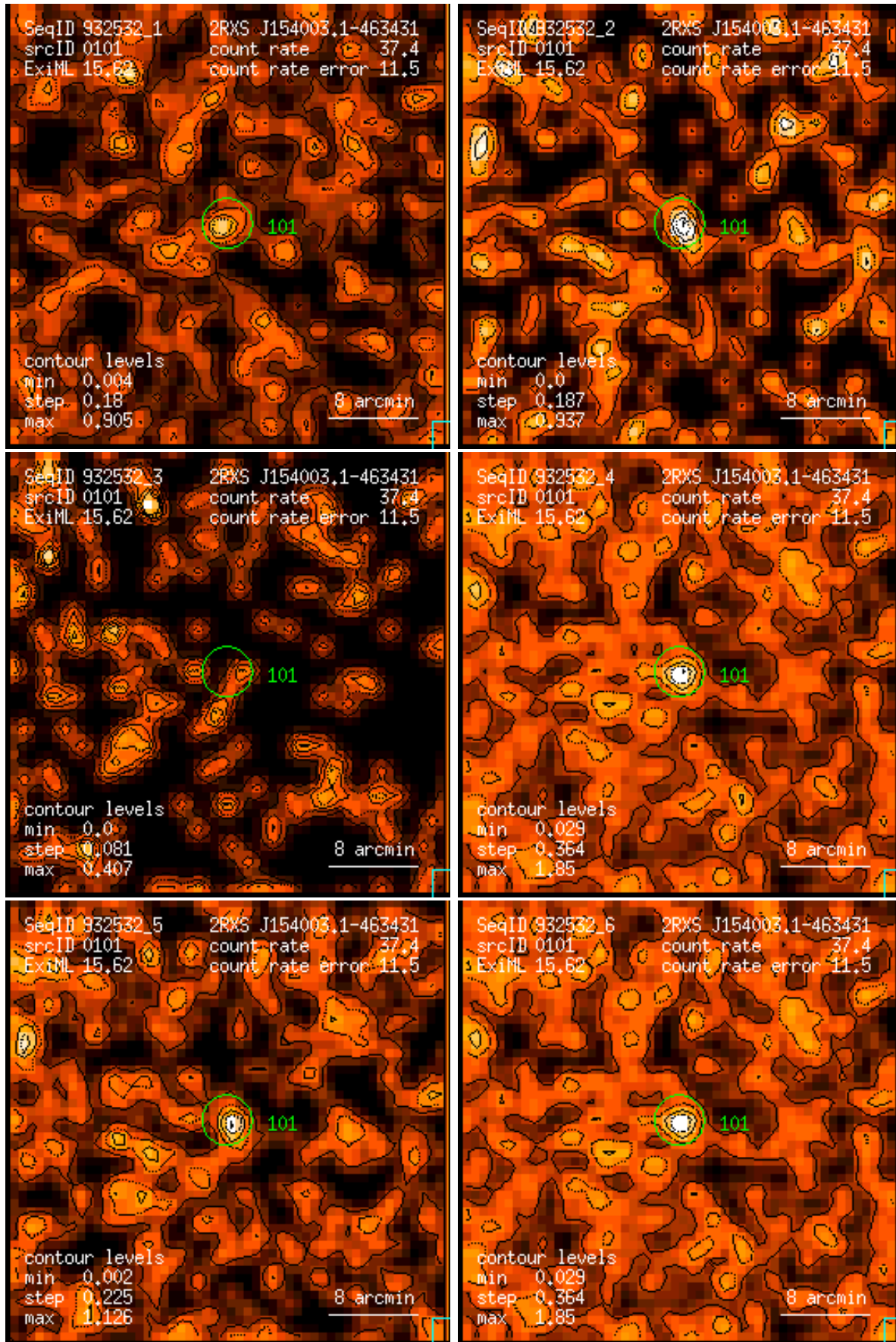
Figure 101: RASS 932532: detection 0101: band rate images, Gaussian filter: (1) PSPC channels 11 – 41, (2) 52 – 90, (3) 91 – 201, (4) 11 – 235, (5) 52 – 201, (6) 11 – 201. Broad band rates in counts/ks. Band rate contour levels in counts/ks/arcmin 2 .
