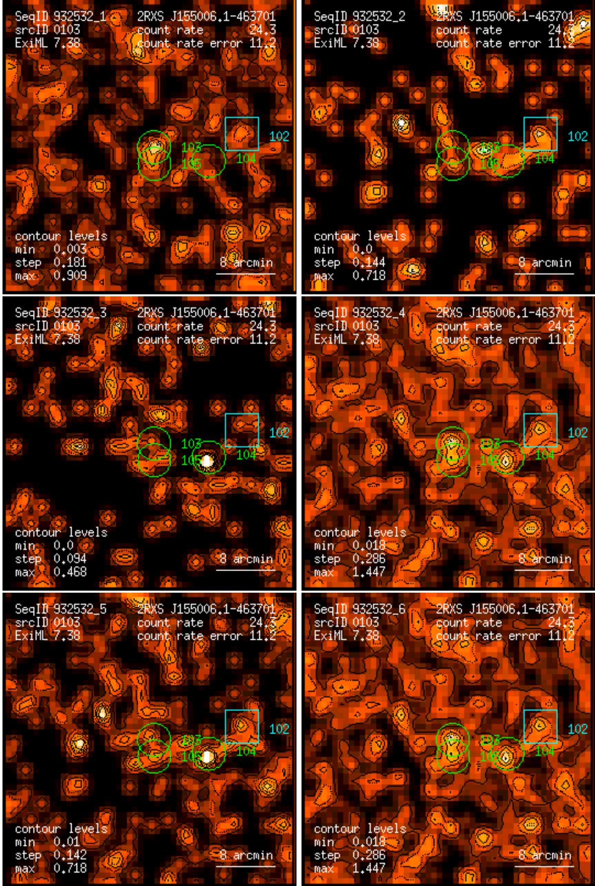
Figure 103: RASS 932532: detection 0103: band rate images, Gaussian filter: (1) PSPC channels 11 – 41, (2) 52 – 90, (3) 91 – 201, (4) 11 – 235, (5) 52 – 201, (6) 11 – 201. Broad band rates in counts/ks. Band rate contour levels in counts/ks/arcmin 2 .
