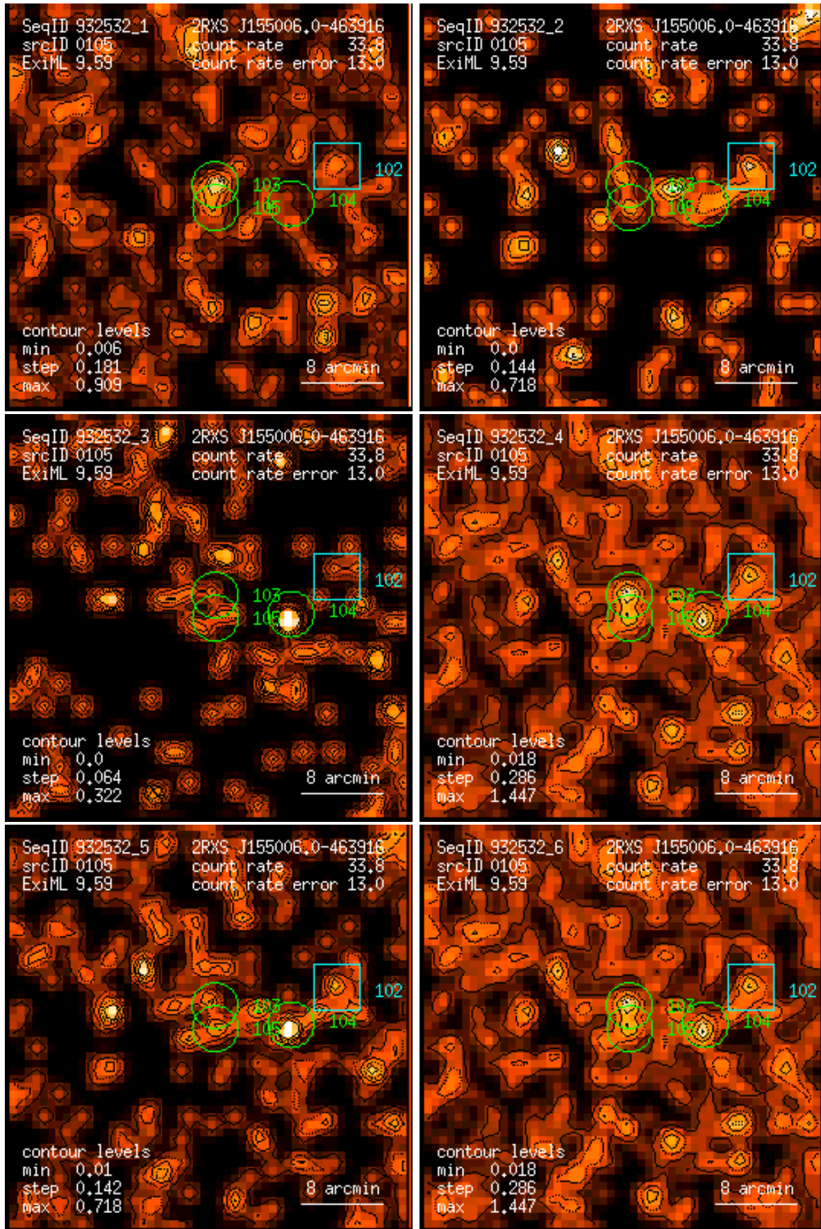
Figure 105: RASS 932532: detection 0105: band rate images, Gaussian filter: (1) PSPC channels 11 – 41, (2) 52 – 90, (3) 91 – 201, (4) 11 – 235, (5) 52 – 201, (6) 11 – 201. Broad band rates in counts/ks. Band rate contour levels in counts/ks/arcmin 2 .
