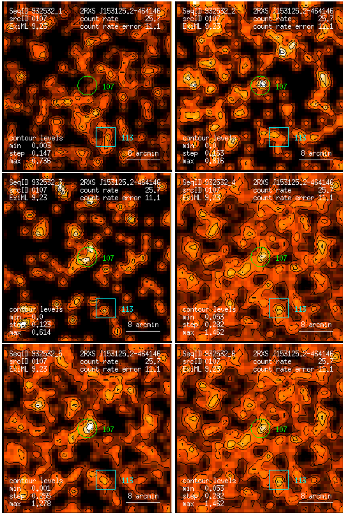
Figure 107: RASS 932532: detection 0107: band rate images, Gaussian filter: (1) PSPC channels 11 – 41, (2) 52 – 90, (3) 91 – 201, (4) 11 – 235, (5) 52 – 201, (6) 11 – 201. Broad band rates in counts/ks. Band rate contour levels in counts/ks/arcmin 2 .
