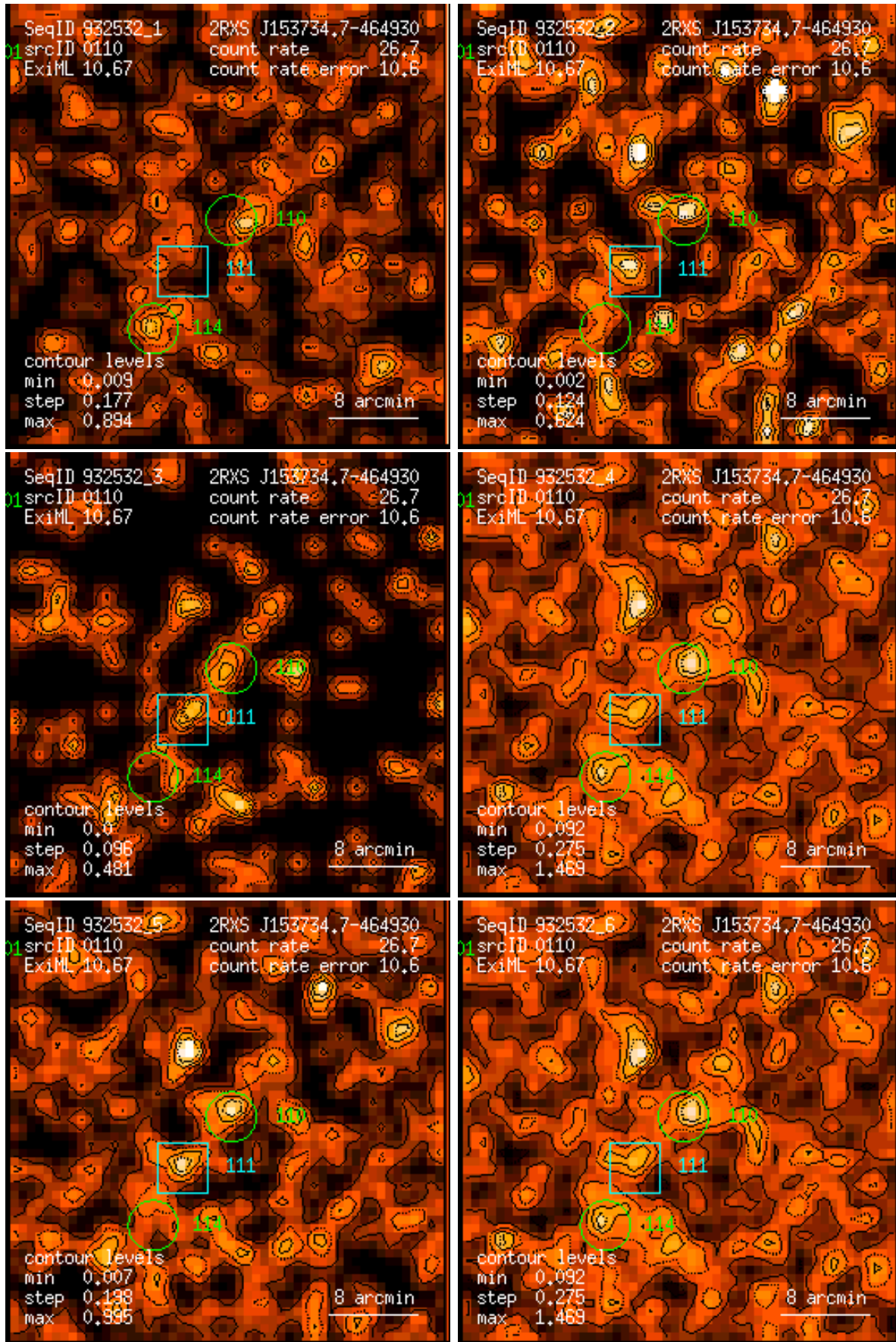
Figure 110: RASS 932532: detection 0110: band rate images, Gaussian filter: (1) PSPC channels 11 – 41, (2) 52 – 90, (3) 91 – 201, (4) 11 – 235, (5) 52 – 201, (6) 11 – 201. Broad band rates in counts/ks. Band rate contour levels in counts/ks/arcmin 2 .
