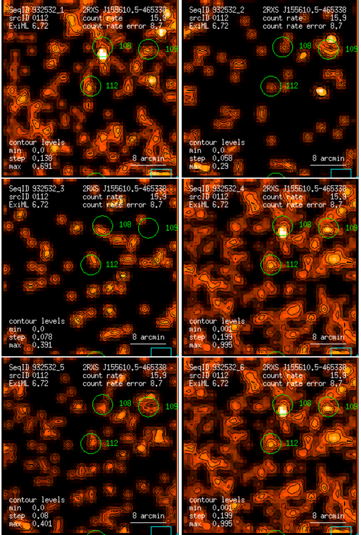
Figure 112: RASS 932532: detection 0112: band rate images, Gaussian filter: (1) PSPC channels 11 – 41, (2) 52 – 90, (3) 91 – 201, (4) 11 – 235, (5) 52 – 201, (6) 11 – 201. Broad band rates in counts/ks. Band rate contour levels in counts/ks/arcmin 2 .
