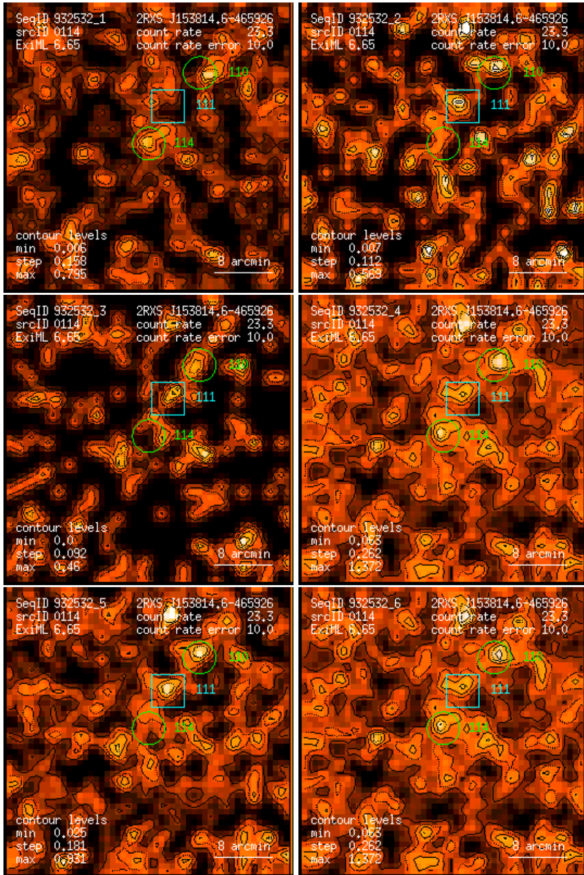
Figure 114: RASS 932532: detection 0114: band rate images, Gaussian filter: (1) PSPC channels 11 – 41, (2) 52 – 90, (3) 91 – 201, (4) 11 – 235, (5) 52 – 201, (6) 11 – 201. Broad band rates in counts/ks. Band rate contour levels in counts/ks/arcmin 2 .
