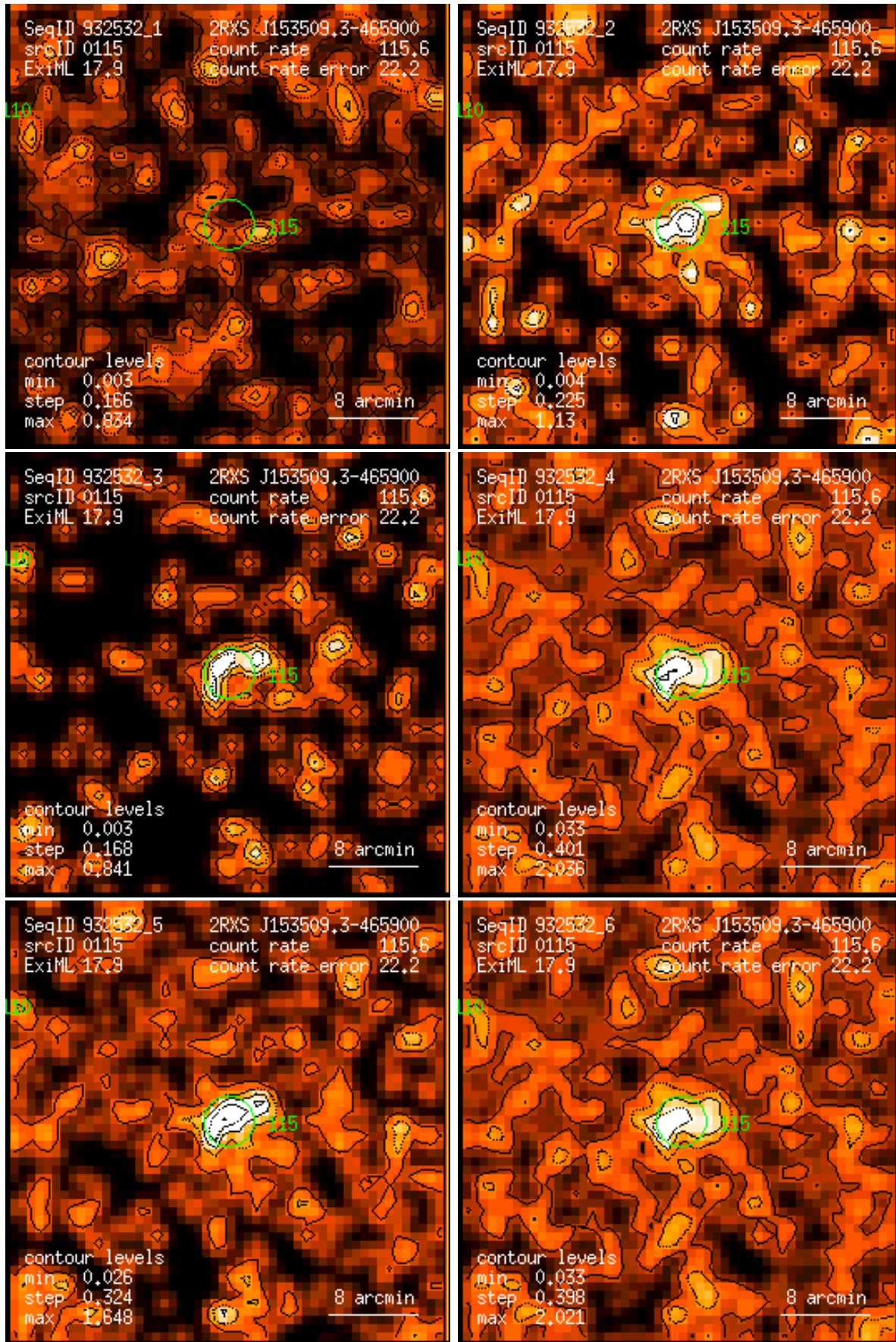
Figure 115: RASS 932532: detection 0115: band rate images, Gaussian filter: (1) PSPC channels 11 – 41, (2) 52 – 90, (3) 91 – 201, (4) 11 – 235, (5) 52 – 201, (6) 11 – 201. Broad band rates in counts/ks. Band rate contour levels in counts/ks/arcmin 2 .
