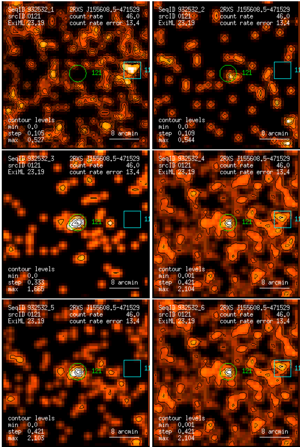
Figure 121: RASS 932532: detection 0121: band rate images, Gaussian filter: (1) PSPC channels 11 – 41, (2) 52 – 90, (3) 91 – 201, (4) 11 – 235, (5) 52 – 201, (6) 11 – 201. Broad band rates in counts/ks. Band rate contour levels in counts/ks/arcmin 2 .
