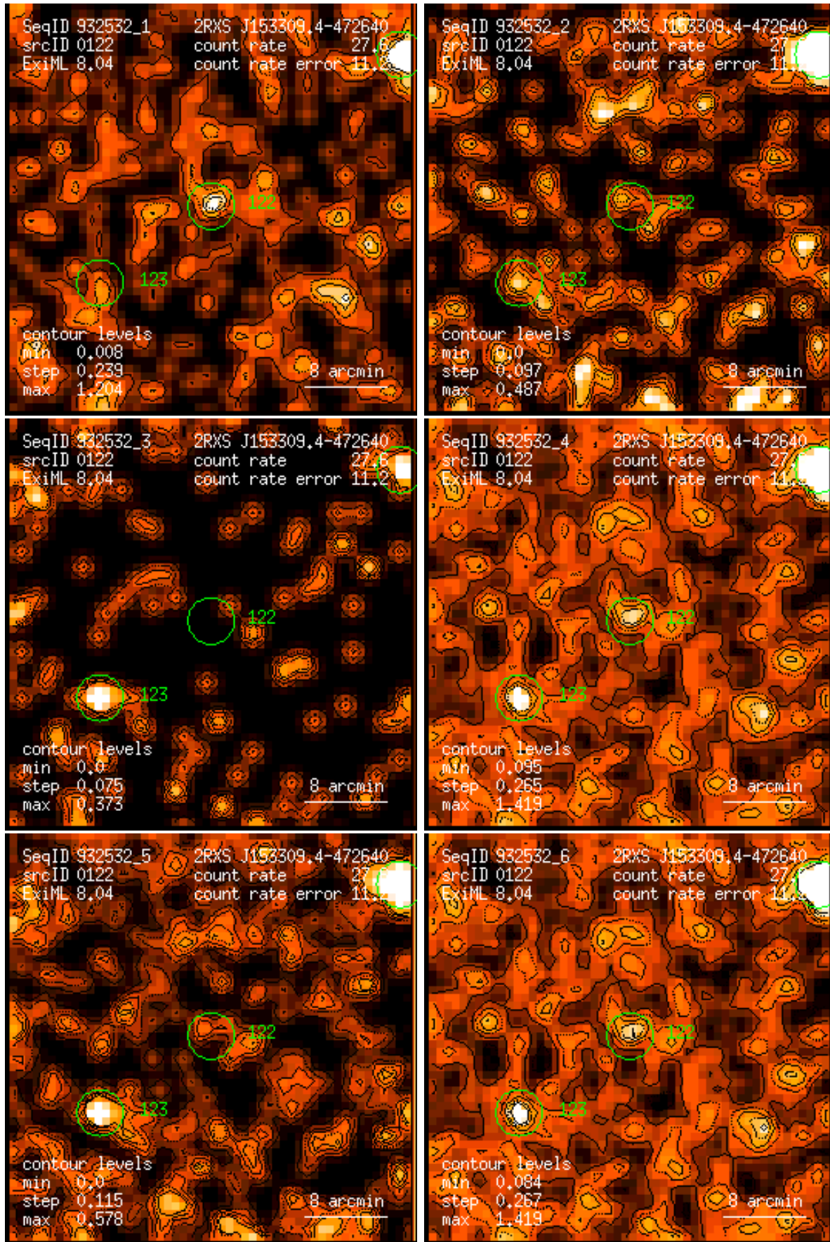
Figure 122: RASS 932532: detection 0122: band rate images, Gaussian filter: (1) PSPC channels 11 – 41, (2) 52 – 90, (3) 91 – 201, (4) 11 – 235, (5) 52 – 201, (6) 11 – 201. Broad band rates in counts/ks. Band rate contour levels in counts/ks/arcmin 2 .
