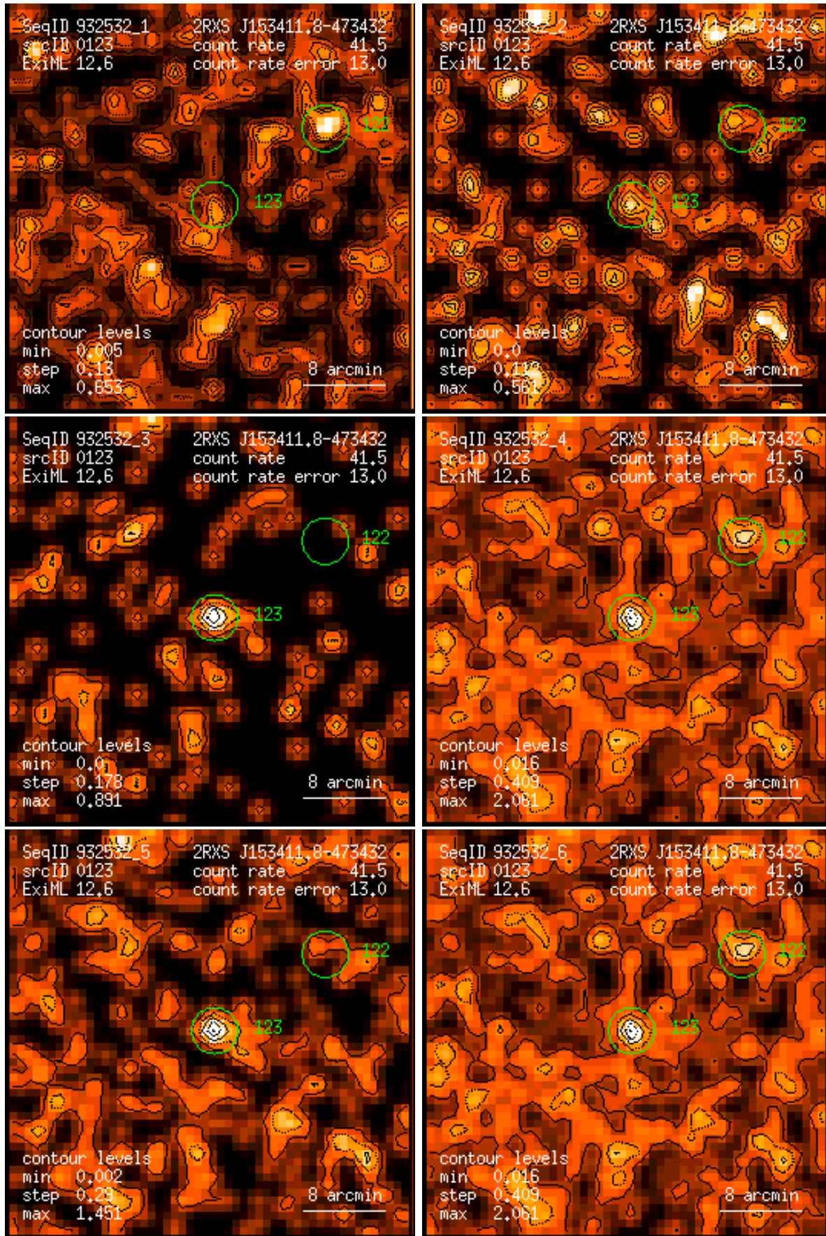
Figure 123: RASS 932532: detection 0123: band rate images, Gaussian filter: (1) PSPC channels 11 – 41, (2) 52 – 90, (3) 91 – 201, (4) 11 – 235, (5) 52 – 201, (6) 11 – 201. Broad band rates in counts/ks. Band rate contour levels in counts/ks/arcmin 2 .
