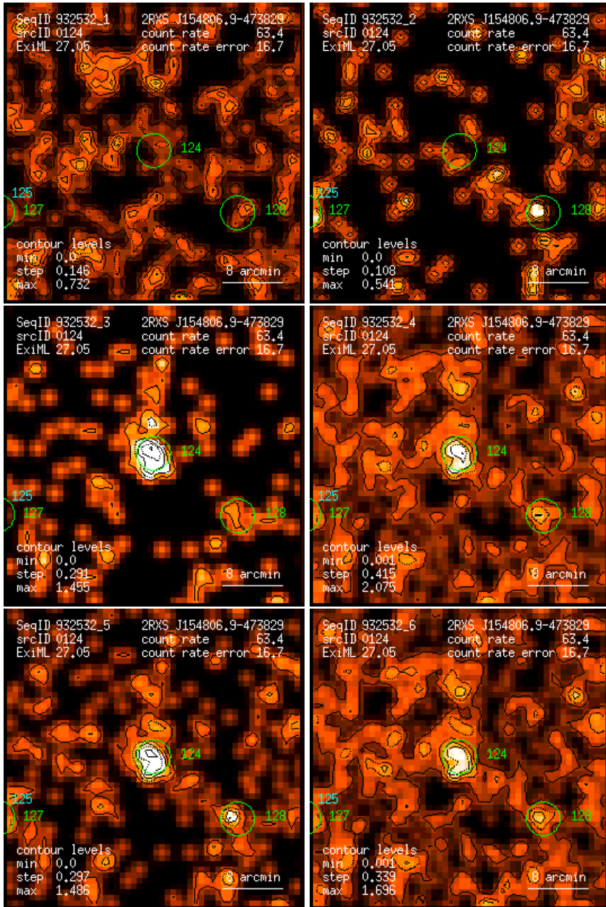
Figure 124: RASS 932532: detection 0124: band rate images, Gaussian filter: (1) PSPC channels 11 – 41, (2) 52 – 90, (3) 91 – 201, (4) 11 – 235, (5) 52 – 201, (6) 11 – 201. Broad band rates in counts/ks. Band rate contour levels in counts/ks/arcmin 2 .
