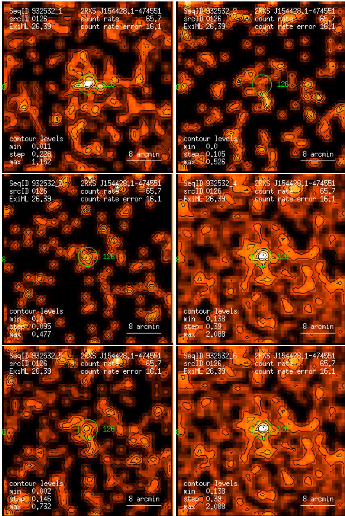
Figure 126: RASS 932532: detection 0126: band rate images, Gaussian filter: (1) PSPC channels 11 – 41, (2) 52 – 90, (3) 91 – 201, (4) 11 – 235, (5) 52 – 201, (6) 11 – 201. Broad band rates in counts/ks. Band rate contour levels in counts/ks/arcmin 2 .
