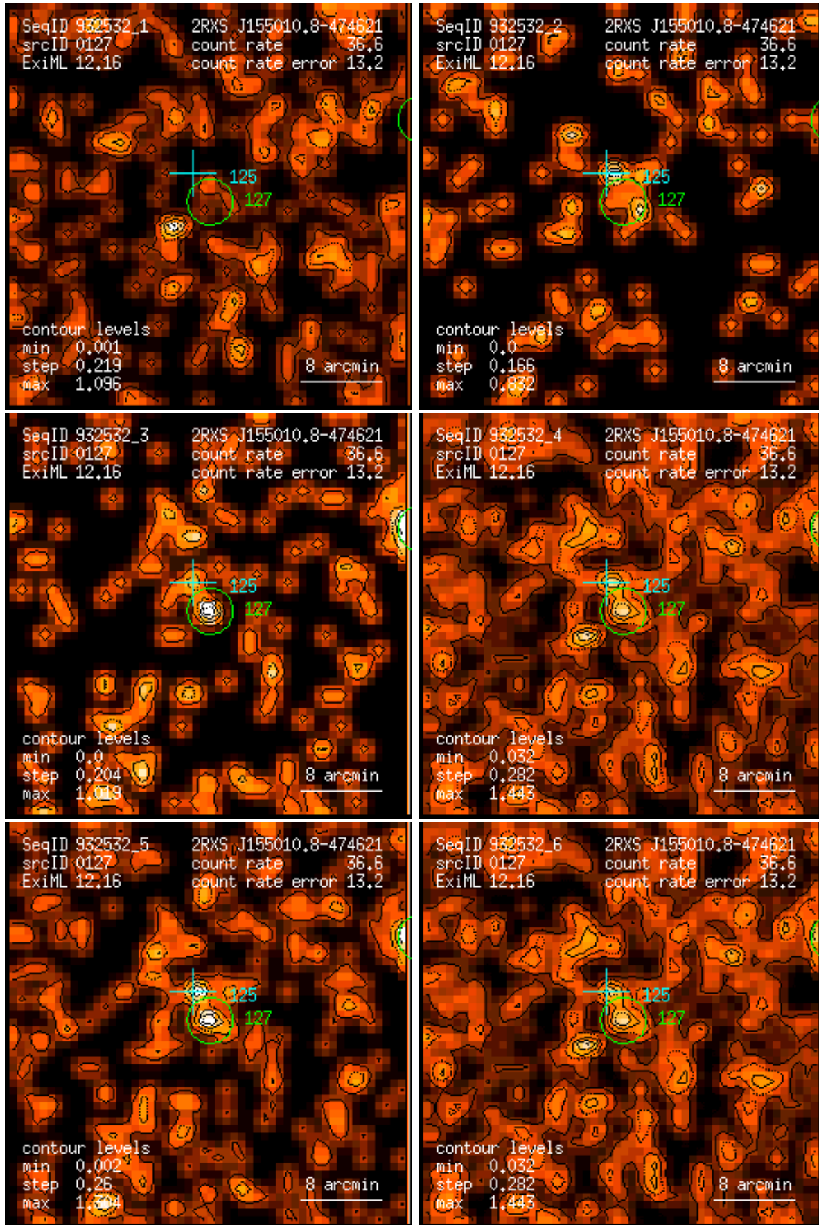
Figure 127: RASS 932532: detection 0127: band rate images, Gaussian filter: (1) PSPC channels 11 – 41, (2) 52 – 90, (3) 91 – 201, (4) 11 – 235, (5) 52 – 201, (6) 11 – 201. Broad band rates in counts/ks. Band rate contour levels in counts/ks/arcmin 2 .
